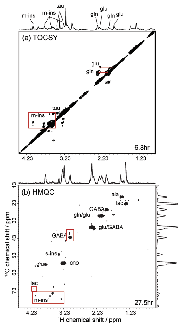
Fig. 3 (a) ^1\text{H} – ^1\text{H} TOCSY and (b) ^1\text{H} – ^{13}\text{C} HMQC HR \mu MAS spectrum of a [3\text{-}^{13}\text{C}]\text{lactate} infused brain biopsy, demonstrating the feasibility of performing homonuclear and heteronuclear 2D experiments with HR \mu MAS. See the ESI† for NMR experimental details.
