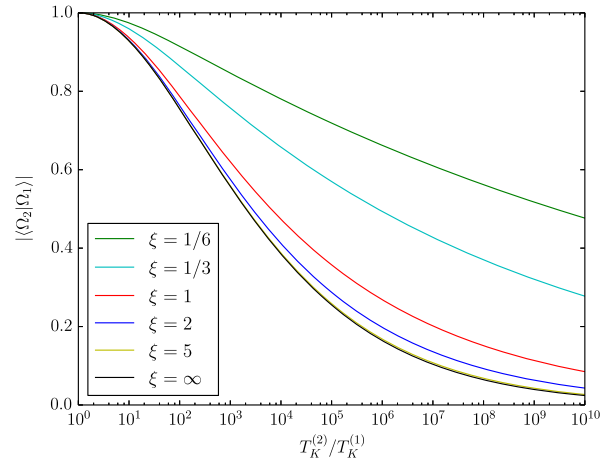
FIG. 2 (color online). Theoretical result for the overlap for various anisotropies as a function of the ratio T_K^{(2)}/T_K^{(1)} . The isotropic Kondo problem then corresponds to \xi = \infty . Note the extreme values on the x axis.
