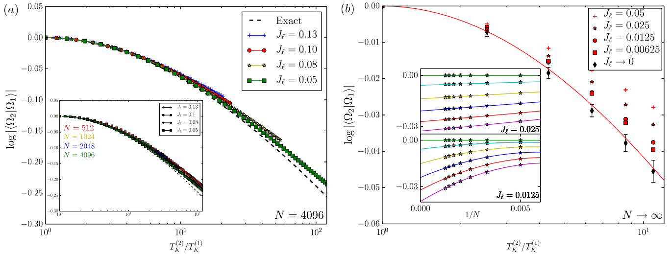
FIG. 3 (color online). Numerical checks of the main result (8). Note that the comparison between numerical and field theory results does not involve any free parameter. (a) Measures of the overlap in the free-fermion Toulouse case \xi = 1 , modeled by a spinless noninteracting resonant level, tunnel coupled with parameter J_\ell to two metallic reservoirs with N = 4096 sites each. The dashed line is the analytical result, with T_K \propto J_\ell^2 . Inset: finite size scaling. (b) DMRG results for the overlap in the interacting case \xi = 1/3 , modeled by an XXZ spin chain with anisotropy \Delta = -1/\sqrt{2} and N sites, with an extra site at the edge characterized by a weak link J_\ell , corresponding to the impurity. The numerical results for N = 200, \dots, 800 are extrapolated in the thermodynamic limit N \rightarrow \infty . The red line is the analytical result, with T_K \propto J_\ell^{4/3} , and the black symbols correspond to the extrapolation J_\ell \rightarrow 0 . Inset: examples of finite size extrapolations for fixed J_\ell \equiv J_\ell^{(1)} and different values of J_\ell^{(2)} .
