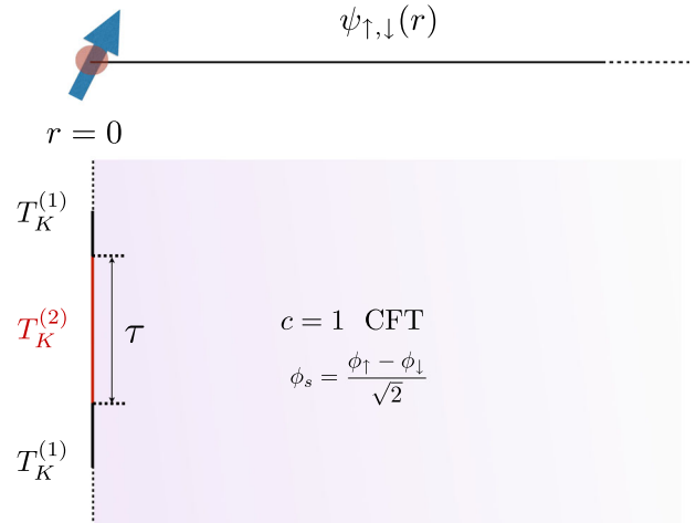
FIG. 1 (color online). The overlap |\langle \Omega_2 | \Omega_1 \rangle| can be extracted from the partition function of the system with the insertion of a Kondo impurity and two different values of the coupling. In this picture, the boundary condition corresponds to the spin impurity while the bulk describes a critical statistical mechanics problem associated with the spin mode \phi_s .
