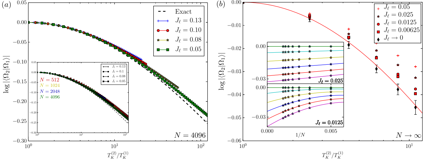
FIG. 3 (color online). Numerical checks of the main result (8). Note that the comparison between numerical and field theory results does not involve any free parameter. (a) Measures of the overlap in the free-fermion Toulouse case \xi = 1 , modeled by a spinless noninteracting resonant level, tunnel coupled with parameter J_\ell to two metallic reservoirs with N = 4096 sites each. The dashed line is the analytical result, with T_K \propto J_\ell^2 . Inset: finite size scaling. (b) DMRG results for the overlap in the interacting case \xi = 1/3 , modeled by an XXZ spin chain with anisotropy \Delta = -1/\sqrt{2} and N sites, with an extra site at the edge characterized by a weak link J_\ell , corresponding to the impurity. The numerical results for N = 200, \dots, 800 are extrapolated in the thermodynamic limit N \rightarrow \infty . The red line is the analytical result, with T_K \propto J_\ell^{4/3} , and the black symbols correspond to the extrapolation J_\ell \rightarrow 0 . Inset: examples of finite size extrapolations for fixed J_\ell \equiv J_\ell^{(1)} and different values of J_\ell^{(2)} .
