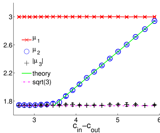
FIG. 3: The first, second and third largest eigenvalues \mu_1 , \mu_2 and |\mu_3| respectively of B as functions of c_{\text{in}} - c_{\text{out}} . The third eigenvalue is complex, so we plot its modulus. Values are averaged over 20 networks of size n = 10^5 and average degree c = 3 . The green line in the figure represents \mu_c = (c_{\text{in}} - c_{\text{out}})/2 , and the horizontal lines are c and \sqrt{c} respectively. The second eigenvalue \mu_2 is well-separated from the bulk throughout the detectable regime.
