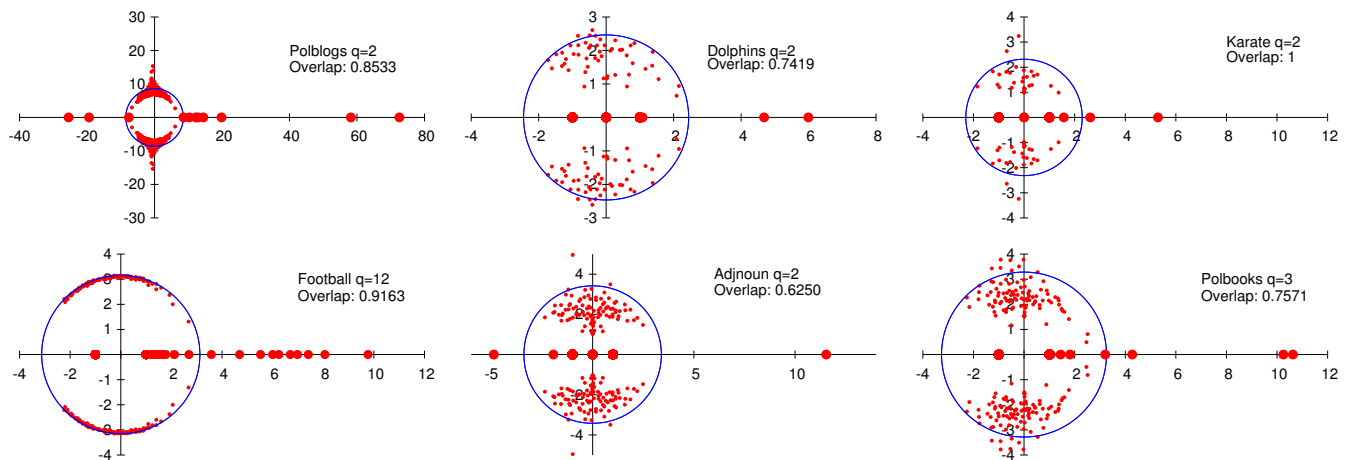
FIG. 6: Spectrum of the non-backtracking matrix in the complex plane for some commonly used benchmarks for community detection in real networks taken from [29–34]. The radius of the circle is the square root of the largest eigenvalue, which is a heuristic estimate of the bulk of the spectrum. The overlap is computed using the signs of the second eigenvector for the networks with two communities, and using k -means for those with three and more communities. The non-backtracking operator detects communities in all these networks, with an overlap comparable to the performance of other spectral methods. As in the case of synthetic networks generated by the stochastic block model, the number of real eigenvalues outside the bulk appears to be a good indicator of the number q of communities.
