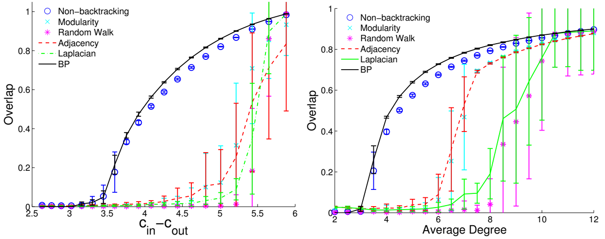
FIG. 4: The accuracy of spectral algorithms based on different linear operators, and of belief propagation, for two groups of equal size. On the left, we vary c_{\text{in}} - c_{\text{out}} while fixing the average degree c = 3 ; the detectability transition given by (1) occurs at c_{\text{in}} - c_{\text{out}} = 2\sqrt{3} \approx 3.46 . On the right, we set c_{\text{out}}/c_{\text{in}} = 0.3 and vary c ; the detectability transition is at c \approx 3.45 . Each point is averaged over 20 instances with n = 10^5 . Our spectral algorithm based on the non-backtracking matrix B achieves an accuracy close to that of BP, and both remain large all the way down to the transition. Standard spectral algorithms based on the adjacency matrix, modularity matrix, the Laplacian, and the random walk matrix fail well above the transition, doing no better than chance.
