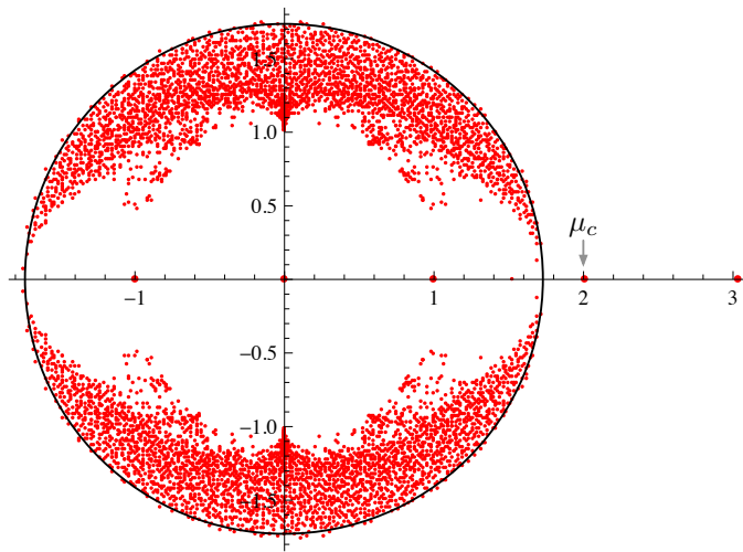
FIG. 2: The spectrum of the non-backtracking matrix B for a network generated by the block model with same parameters as in Fig. 1. The leading eigenvalue is at c = 3 , the second eigenvalue is close to \mu_c = (c_{\text{in}} - c_{\text{out}})/2 = 2 , and the bulk of the spectrum is confined to the disk of radius \sqrt{c} = \sqrt{3} . Since \mu_c is outside the bulk, a spectral algorithm that labels vertices according to the sign of B 's second eigenvector (summed over the incoming edges at each vertex) labels the majority of vertices correctly.
