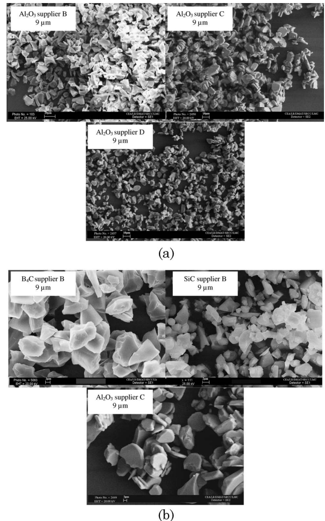
Fig. 2. (a) Typical SEM pictures of 9 \mu\text{m} \text{Al}_2\text{O}_3 particles. (b) SEM pictures of 9 \mu\text{m} \text{Al}_2\text{O}_3 , SiC, and \text{B}_4\text{C} particles.
