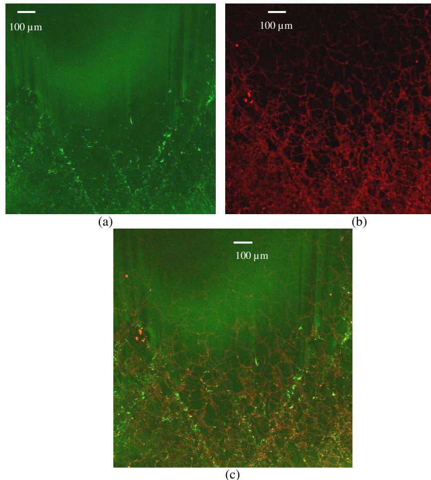
Fig. 4. Sample D2 – Confocal microscopy image of the surface in the MRF dimple on an area of 1.5 \times 1.5 \text{ mm}^2 , approximately 50 \mu\text{m} removed by MRF between border of the dimple and top of the figure. Same area measured in reflection at 458 nm (a), fluorescence in the 435-661nm spectral band for an excitation wavelength of 405 nm (b) and superposition of the two images (c) – 63 x objective
