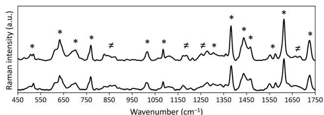
Figure 3. FT-Raman comparison of nanotubular and microcrystalline forms. (A) FT-Raman spectra of 10%w/w lanreotide nanotubes gel (top graph) and of centrifuged microcrystals of derivative 4 (bottom graph). The symbols '*' and '#' respectively indicate similar and differing peaks.
