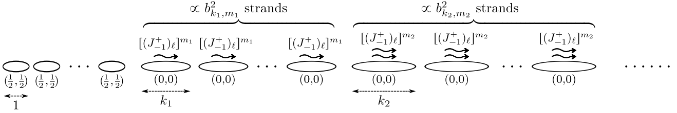
Figure 5: The dual CFT state for the superstrata geometries in Section 5. The symbol [(J_{-1}^+)_{\ell}]^m above a (0,0) strand means that we act m times by the operator (J_{-1}^+)_{\ell} on the ground state of the CFT on the strand. The wavy arrows represent the non-vanishing momentum modes excited on the strand. The number of strands of the same type is \mathcal{O}(N) , meaning that our solution represents a finite non-linear deformation around the AdS_3 \times S^3 background. For the precise numbers of each type of strand, see (7.8).
