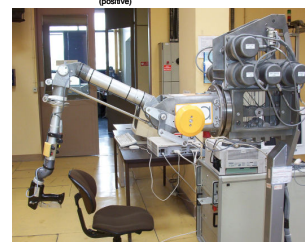
Figure 3 – Key actuator principle of the master arm MA23 CEA/La Calhène
