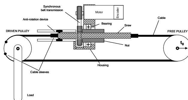
Figure 5 - Initial design of a screw-nut cable actuator
