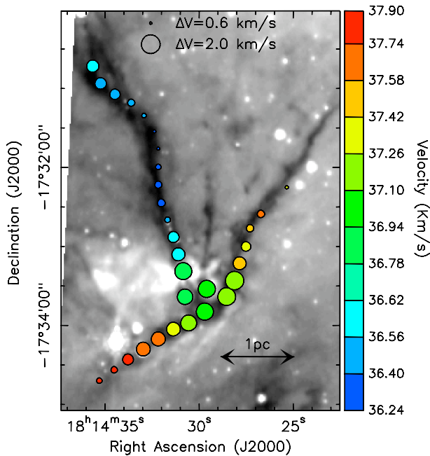
Fig. 4. Spitzer 8 \mu m image of SDC13 in grey scale on top of which we symbolised the results of the N_2H^+(1-0) HFS fitting as circles. The colour of the symbols indicate the gas velocity while their sizes indicate the gas velocity dispersion (FWHM).
