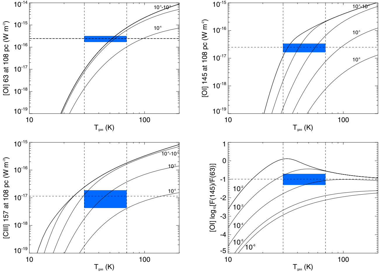
Fig. 2. Predicted [OI] 63 and 145 \mu\text{m} and [C II] 157 \mu\text{m} fine-structure fluxes as a function of the gas temperature. The fourth panel shows the predicted ratio between the [OI] 63 and 145 \mu\text{m} fluxes. The observed ratio is overplotted by the horizontal dashed lines. The total disk gas masses in M_{\odot} are indicated. The blue box encompasses gas temperatures between 30 and 70 K and the observed [OI] at 63 \mu\text{m} , [OI] at 145 \mu\text{m} , [C II] at 157 \mu\text{m} , and the F([\text{OI}]145 \mu\text{m})/F([\text{OI}]63 \mu\text{m}) flux with 3\sigma error bars.
