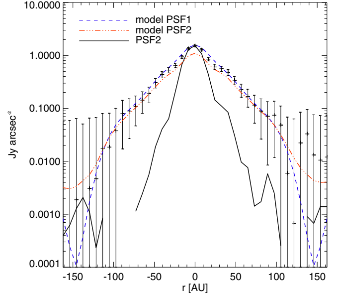
Fig. 8. Fit to the PAH radial emission profile at 8.6\ \mu\text{m} along the major axis obtained with VISIR at the VLT. The same model has been convolved with the observed or theoretical noise-free PSF. The theoretical PSF fits the core of the observed function. The model succeeded in fitting the profile.
