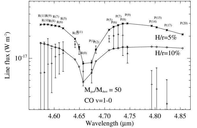
Fig. 16. Some modeled CO fundamental ro-vibrational fluxes compared with the observed fluxes taken from Brittain et al. (2007). The error bars are 3\sigma uncertainties. The identification of the lines are labelled. The two models have a gas-to-dust-mass ratio of 50. The opening angles are 5% and 10%.
