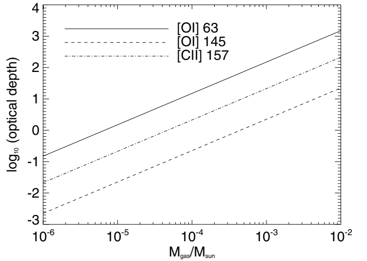
Fig. 4. [O I] 63 and 145 \mu m and [C II] 157 \mu m line optical depths as a function of the gas disk mass at T_{\text{gas}} = 60 \text{ K} .
