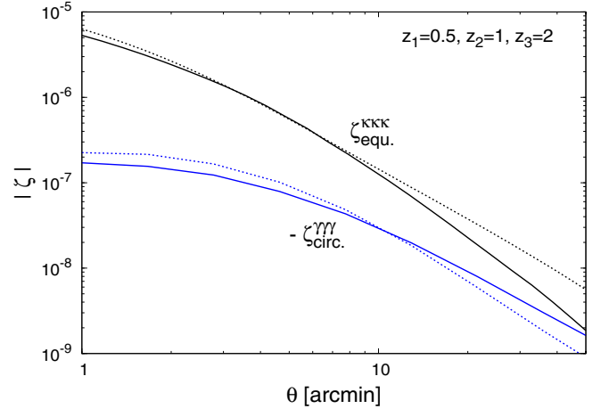
Fig. D.1. Convergence and shear three point correlations \zeta_{\text{equ.}}^{KKK} and \zeta_{\text{circ.}}^{\gamma\gamma\gamma} , as a function of the angular scale \theta , for the redshift triplet z_1 = 0.5, z_2 = 1, z_3 = 2 . We show the predictions from the model of Valageas et al. (2012a,b) (solid lines) and from the hierarchical ansatz (18) (dotted lines). Because \zeta_{\text{circ.}}^{\gamma\gamma\gamma} is negative we plot -\zeta_{\text{circ.}}^{\gamma\gamma\gamma} .
