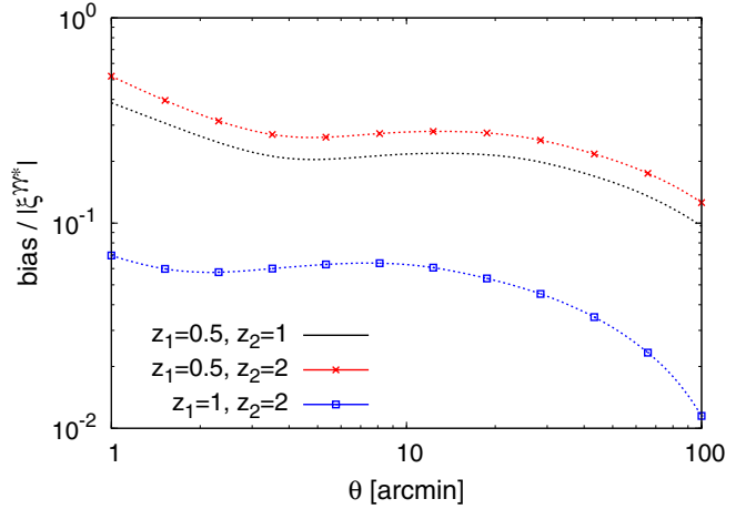
Fig. 12. Relative intrinsic-alignment bias of the weak lensing shear two-point correlation, \xi^I / |\xi^{\gamma\gamma^*}| , as a function of the angular scale \theta , for three pairs of different source redshifts, (z_1, z_2) = (0.5, 1) , (0.5, 2) , and (1, 2) . All total biases are negative.
