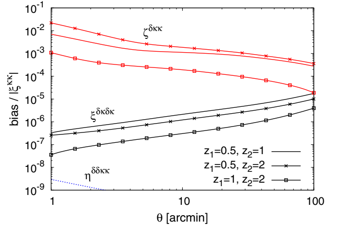
Fig. 3. Same as in Fig. 2, but for pairs of different source redshifts, (z_1, z_2) = (0.5, 1), (0.5, 2) , and (1, 2) . The contribution \eta^{\delta\delta KK} is negative as shown by the dotted line.
