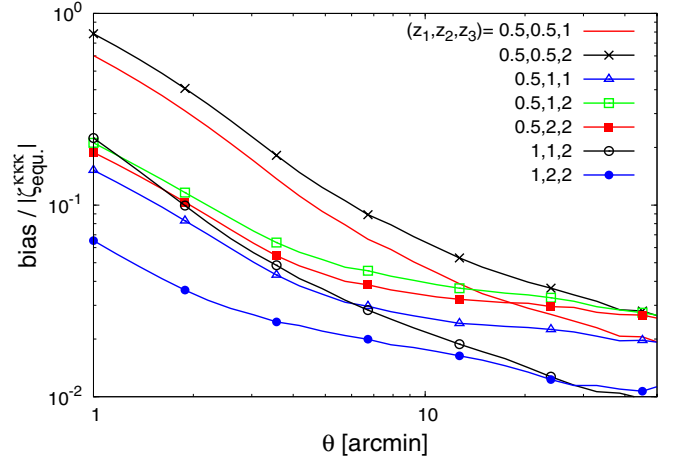
Fig. 8. Relative source-lens clustering bias of the equilateral weak lensing convergence three-point correlation \zeta_{\text{equ}}^{KKK} , as a function of the angular scale \theta , for a few redshift triplets z_1 \leq z_2 \leq z_3 . All total biases are positive.
