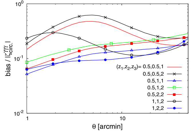
Fig. 10. Relative source-lens clustering bias of the circular weak lensing shear three-point correlation \xi_{\text{circ}}^{\gamma\gamma\gamma} , as a function of the angular scale \theta , for a few redshift triplets z_1 \leq z_2 \leq z_3 . All total biases are positive.
