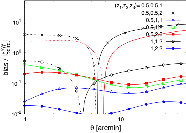
Fig. 14. Relative intrinsic-alignment bias of the circular weak lensing shear three-point correlation \zeta_{\text{circ}}^{\gamma\gamma\gamma} , as a function of the angular scale \theta , for a few redshift triplets z_1 \leq z_2 \leq z_3 .
