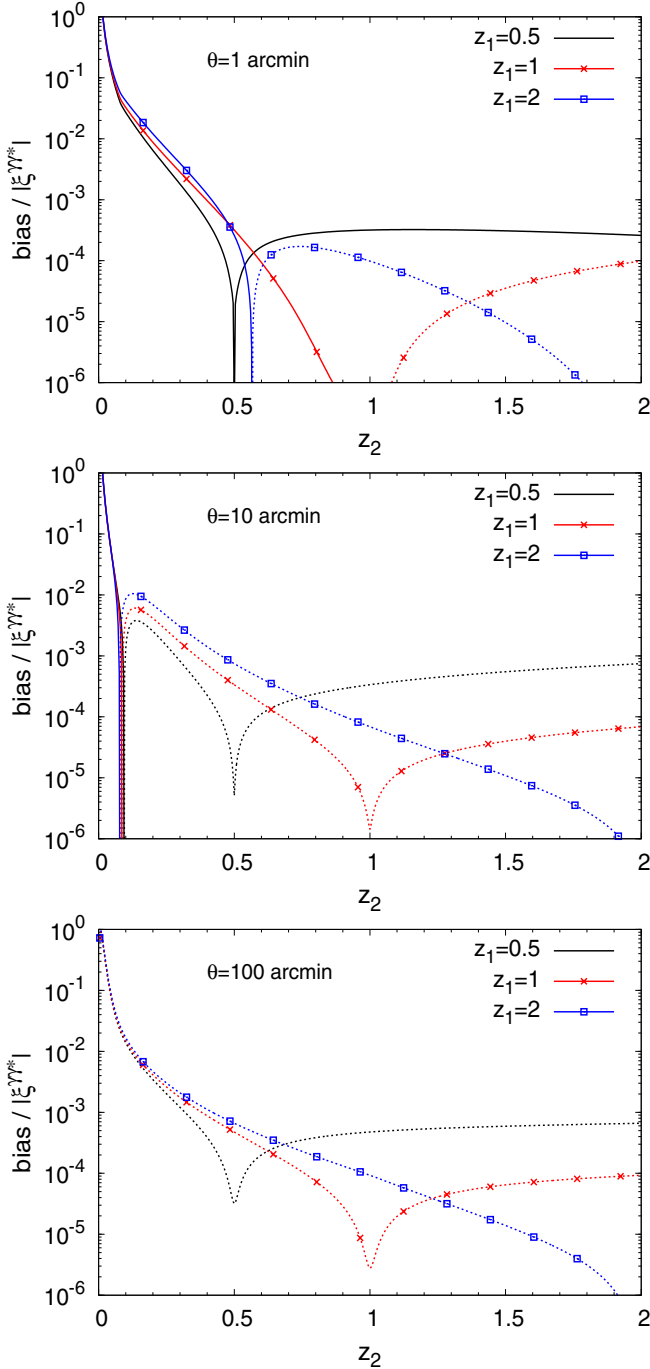
Fig. 7. Relative source-lens clustering bias of the weak lensing shear two-point correlation, (\xi^{\delta\gamma\delta\gamma^*} + \xi^{\delta\gamma\gamma^*})/|\xi^{\gamma\gamma^*}| (we neglect the four-point contribution), as a function of the second galaxy redshift z_2 , for a fixed first galaxy redshift z_1 = 0.5, 1 , or 2 . We consider the angular scales \theta = 1, 10 , and 100 arcmin, from the upper to the lower panels.
