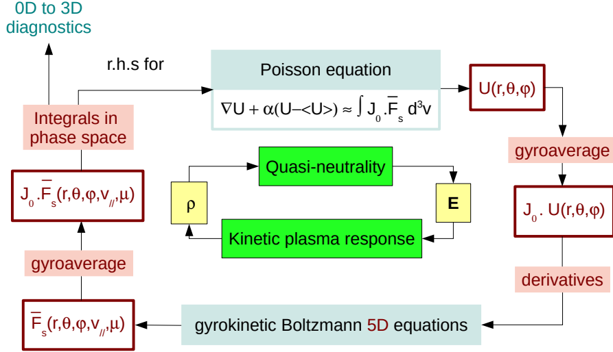
Figure 3: Schematic view of the coupling between the Poisson and Vlasov solvers in the GYSELA code.
