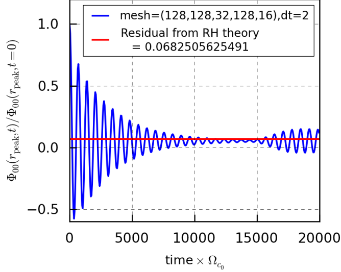
Figure 9: Comparison of the residual value of the (0,0) mode \phi_{00}(r_{\text{peak}}, t) / \phi_{00}(r_{\text{peak}}, t = 0) = A_r where A_r = 1 / (1 + 1.6q^2 / \sqrt{r/R}) = 0.06825 is given by Rosenbluth-Hinton theory. This result corresponds to simulation 1 described in Table 8.
