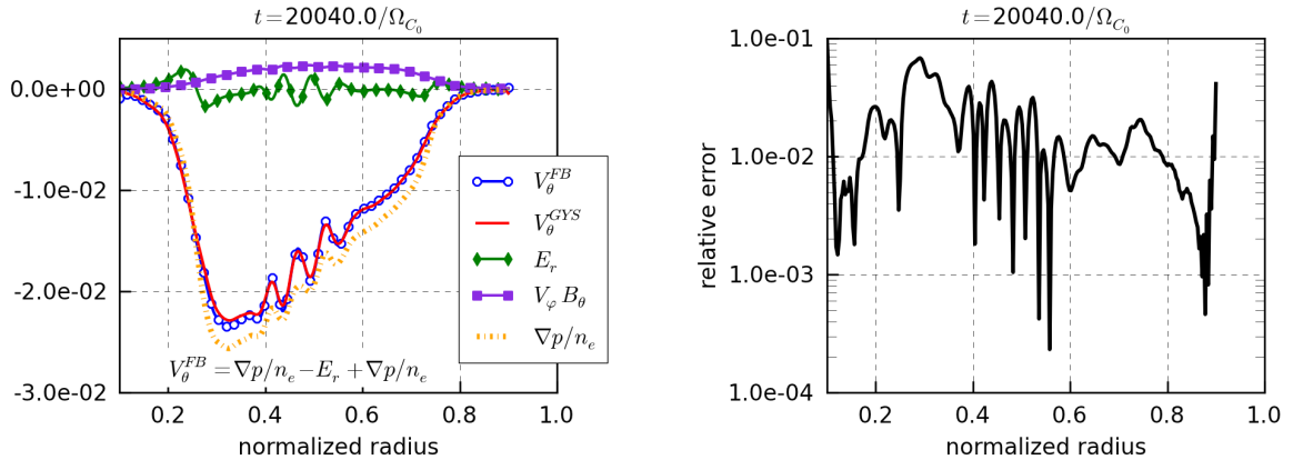
Figure 12: Left: Numerical test of the radial force balance equation (58) at time t = 20040\Omega_{C_0}^{-1} , comparing the poloidal velocity v_\theta^{\text{GYS}} directly computed in the code and v_\theta^{\text{FB}} the sum of the three contributions -E_r , \nabla p / n_e and v_\phi B_\theta . Right: Relative error between both. The parameters used for this simulation are summarized in Table 11.
