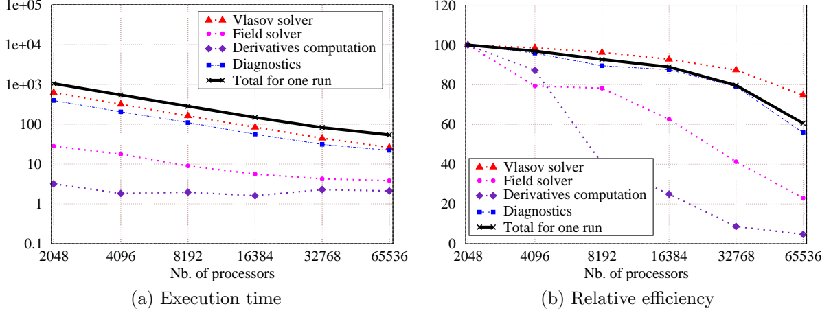
Figure 5: Strong scaling performed on the Curie machine from 2048 to 65536 cores: Execution time (a) and relative efficiency (b) for one GYSELA run of 4 iterations for a mesh (N_r \times N_\theta \times N_\varphi \times N_{v_{G\parallel}} \times N_\mu) = (512 \times 512 \times 128 \times 128 \times 32) with 8 threads and 32 values in \mu direction.
