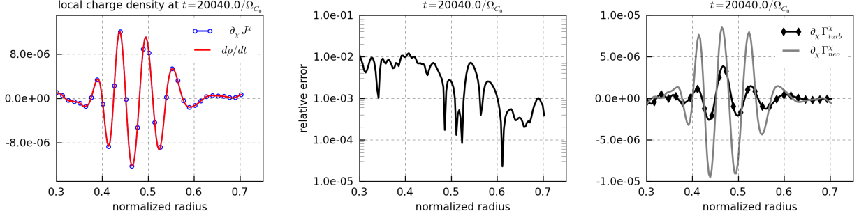
Figure 11: Numerical test of the charge density conservation for simulation defined in Table 11. All the quantities are flux-surface averaged. Left: Comparison of the two terms -\partial_\chi J^\chi and d\rho/dt which must be equivalent according to equation eq.(60). Middle: Relative error (defined as the difference normalized to the quadratic mean). Right: Contribution of the neoclassical and turbulent parts.
