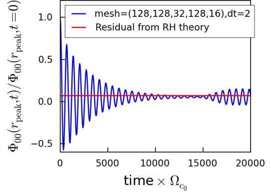
Figure 7: Comparison of the residual value of the (0,0) mode \phi_{00}(r_{\text{peak}}, t)/\phi_{00}(r_{\text{peak}}, t = 0) = A_r where A_r = 1/(1 + 1.6q^2/\sqrt{r/R}) = 0.06825 is given by Rosenbluth-Hinton theory. This result corresponds to simulation 1 described in Table 8.
