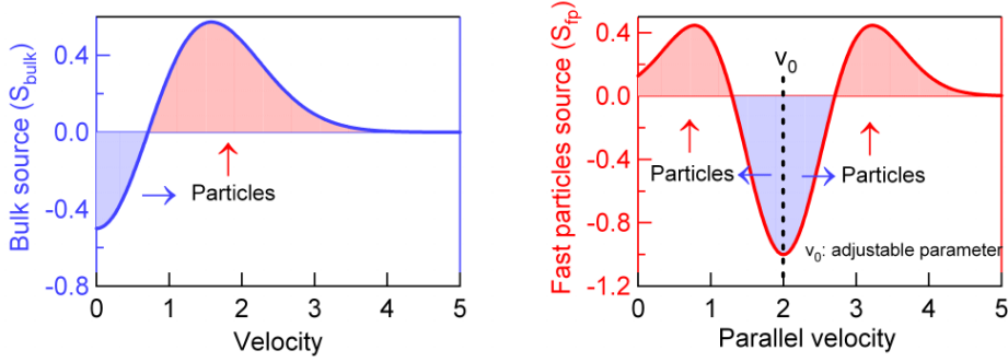
Figure 1: Schematic view of the energetic particle source as a function of the parallel velocity
