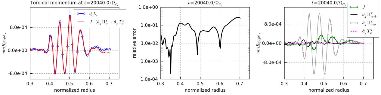
Figure 13: Numerical test for local toroidal momentum conservation for simulation detailed in Table 11. All the quantities are flux-surface averaged. Left: Comparison between \partial_t \mathcal{L}_\varphi and J^X - \partial_\chi \Pi_\varphi^X - T_{\text{pol}}^X which must be equal according to eq.(77). Middle: Relative error (defined here as the difference normalized to the quadratic mean). Right: Detailed contributions of neoclassical and turbulent parts.
