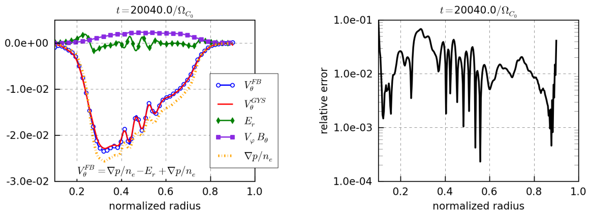
Figure 10: Left: Numerical test of the radial force balance equation (58) at time t = 20040\Omega_{C_0}^{-1} , comparing the poloidal velocity v_\theta^{\text{GYS}} directly computed in the code and v_\theta^{\text{FB}} the sum of the three contributions -E_r , \nabla p / n_e and v_\varphi B_\theta . Right: Relative error between both. The parameters used for this simulation are summarized in Table 11.
