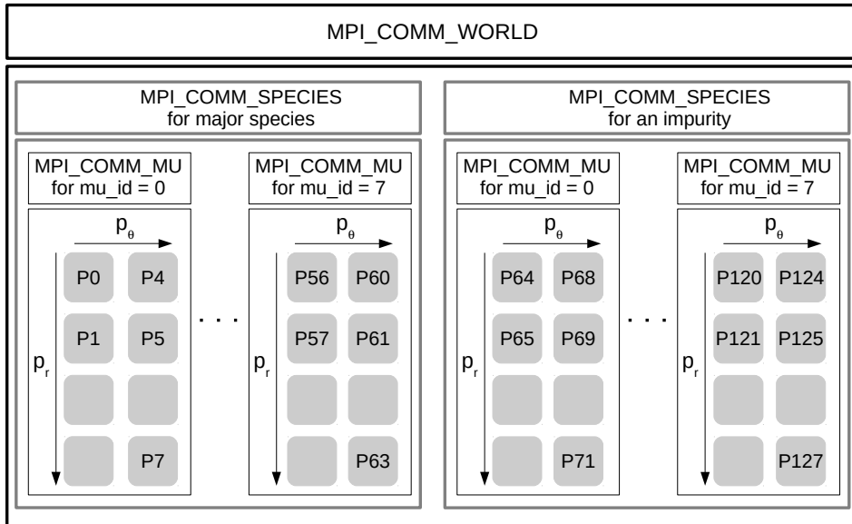
Figure 3: MPLCOMM_WORLD communicator decomposition for two species, 8 values of \mu , p_r = 4 radial sub-domains and p_\theta = 2 sub-domains in the poloidal direction. In this case, the number of MPI processes is equal to 128.
