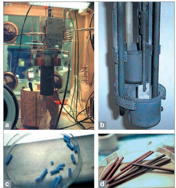
Fig. 137. Nuclearized batch contactor (a and b), and salt prior to contact (c and d) [blue color characteristic of Pu(III)] and after contact (brown color characteristic of lanthanides).
