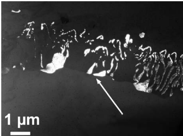
Fig. 64. Carbide precipitation in a superalloy (Haynes 230).
