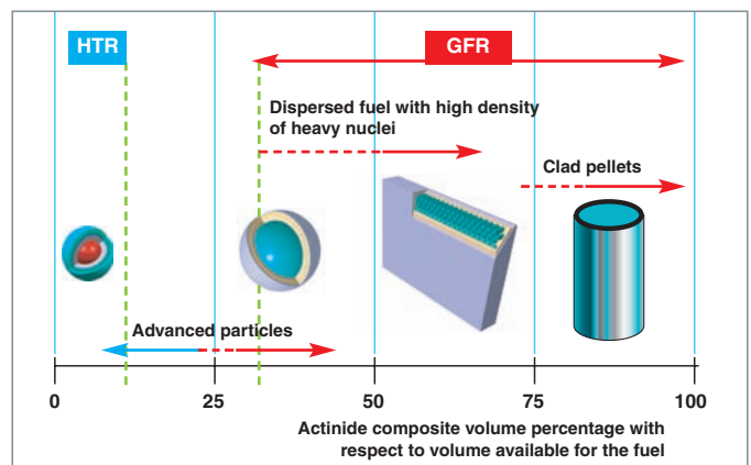
Fig. 120. Candidate concepts for GFR fuel.
