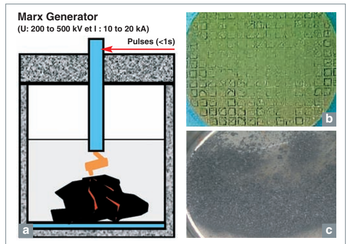
Fig. 129. Basic diagram of the pulsed-current process (a), and image of an SiC honeycomb structure filled with SiC (plate-type fuel), prior to application of pulsed currents (b) and after 30 pulses (c).
