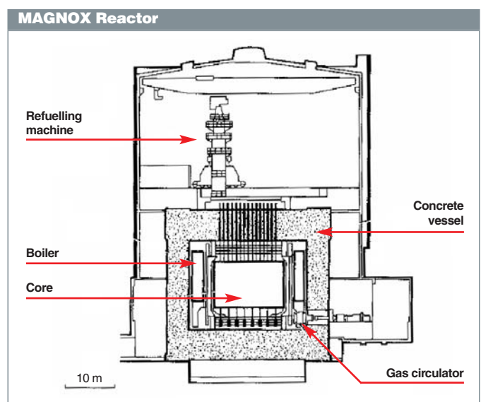
Fig. 10. MAGNOX Reactor.
