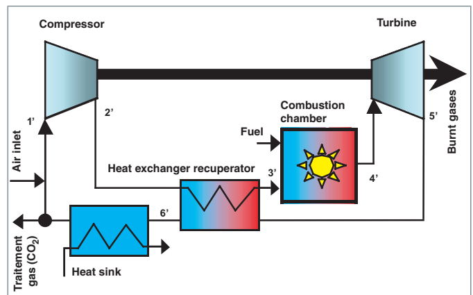
Fig. 75. Semi-open Joule-Brayton cycle with recuperator. The numbers indicate corresponding points in Figures 73 and 74.
