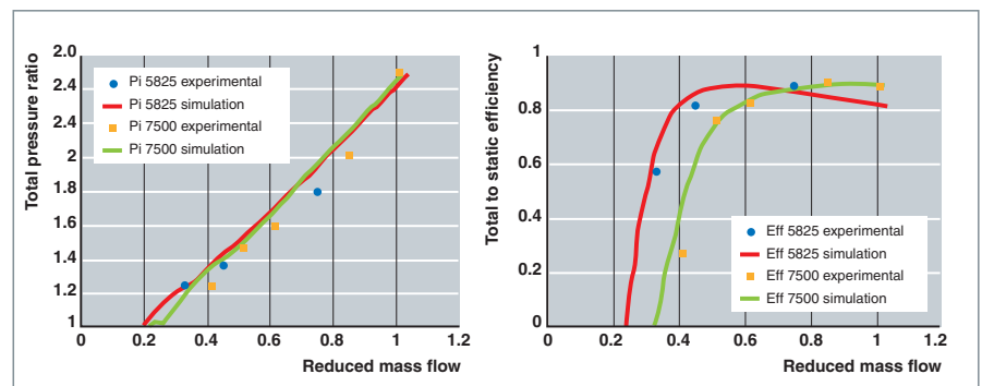
Fig. 78. CEA modeling of a turbomachine: Adimensional comparison of experimental/simulated pressure (left) and isostatic efficiency (right) as a function of mass flow rate.
