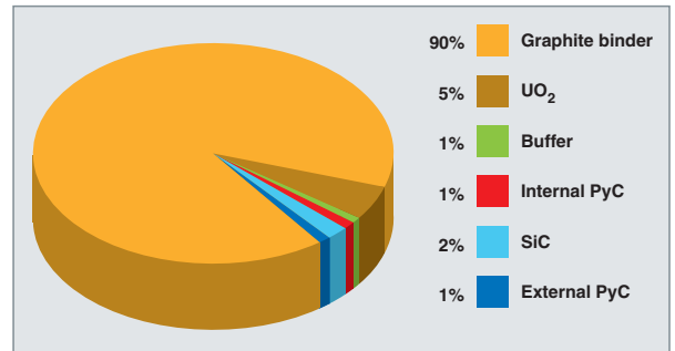
Fig. 51. Composition by weight of an HTR fuel element (pebble or compact).
