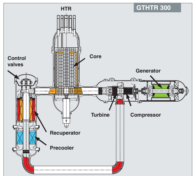
Fig. 25. Japanese GTHTR-300 project.
