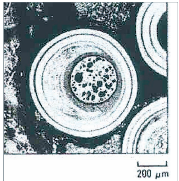
Fig. 68. Amoeba effect observed in coated particle fuel at high temperature. It consists of a displacement of the \text{UO}_2 core in the porous buffer until contacting the internal PyC, possibly leading to rupture of the particle.
