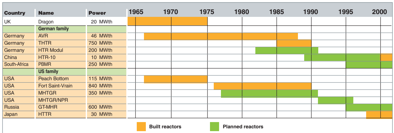
Fig. 21. HTRs worldwide (above) and main characteristics of HTRs built (below).
