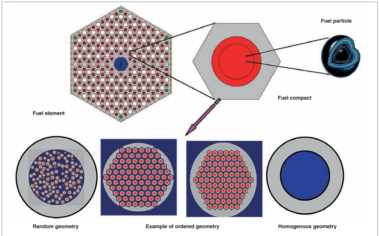
Fig. 41. Example of applications of the TRIPOLI4 code to model HTR particle fuels. Various representations of the random medium have been tested: random distribution, reduced or non-reduced hexagonal structure, cubic structure, homogeneous medium (based on cross sections calculated by APOLLO2). As a general rule, the random distribution of materials in the core should have no impact on the neutronic calculation results if the characteristic size of the
