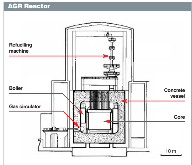
Fig. 11. Cross-section of an AGR.
