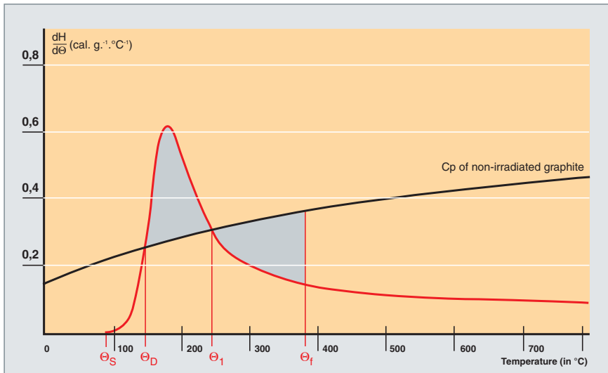
Fig. 15. The Wigner energy spectrum for irradiated graphite at 60 °C having received a neutron fluence of 1.74 \cdot 10^{20} n.cm -2 \phi FG ( i.e. 0.12 displacement per atom).
