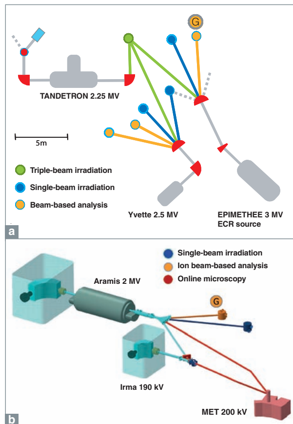
Fig. 113. Basic diagram of the JANNUS irradiation platform. Set of three linear accelerators at the Saclay site (a) and two accelerators + MET in-situ at the CNRS-IN2P3 Orsay site (b).
