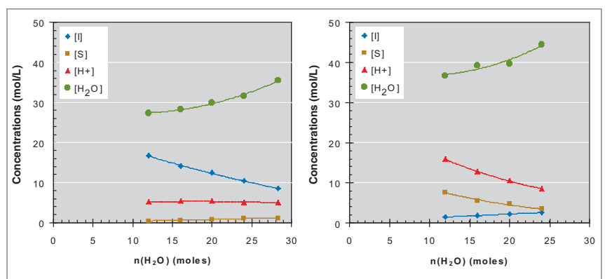
Fig. 96. Total quantities of iodine, sulfur, protons and water measured in the HIx phase (left) and in the sulfuric acid phase (right) obtained by mixing HI/H_2SO_4/I_2/H_2O = 2/1/2/n (molar proportions) at 303 °K.
