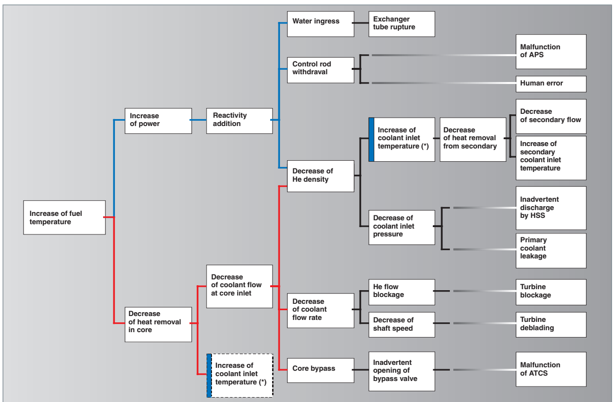
Fig. 103. Simplified tree structure of initiating events leading to an abnormal increase in fuel temperature.
