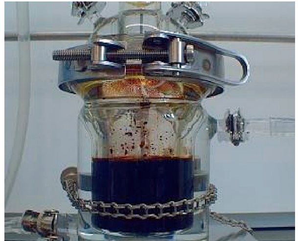
Fig. 95. The B0 reaction vessel built by the Physics and Chemistry Department is used to demonstrate the separation of the phases produced by the Bunsen reaction, and to quantify the composition of the phases in equilibrium (see example in Fig. 96).
