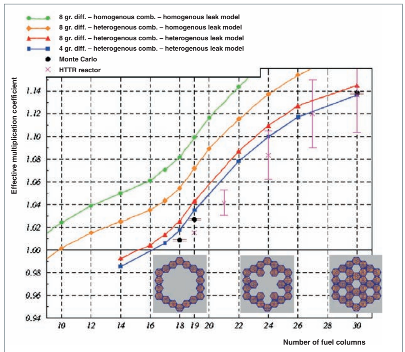
Fig. 39. HTTR reactivity according to number of fuel elements.
