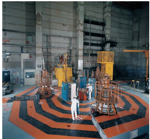
Fig. 4. Reactor hall in the Phénix plant. Located on the Rhone riverbank, the Phénix plant is an integral component of the Marcoule nuclear site (Gard province) and a prototype of the sodium-cooled fast neutron reactor series (RNR-Na). The experimental program mainly concerns the transmutation of actinides, but the experience acquired also benefits research on future nuclear systems.
