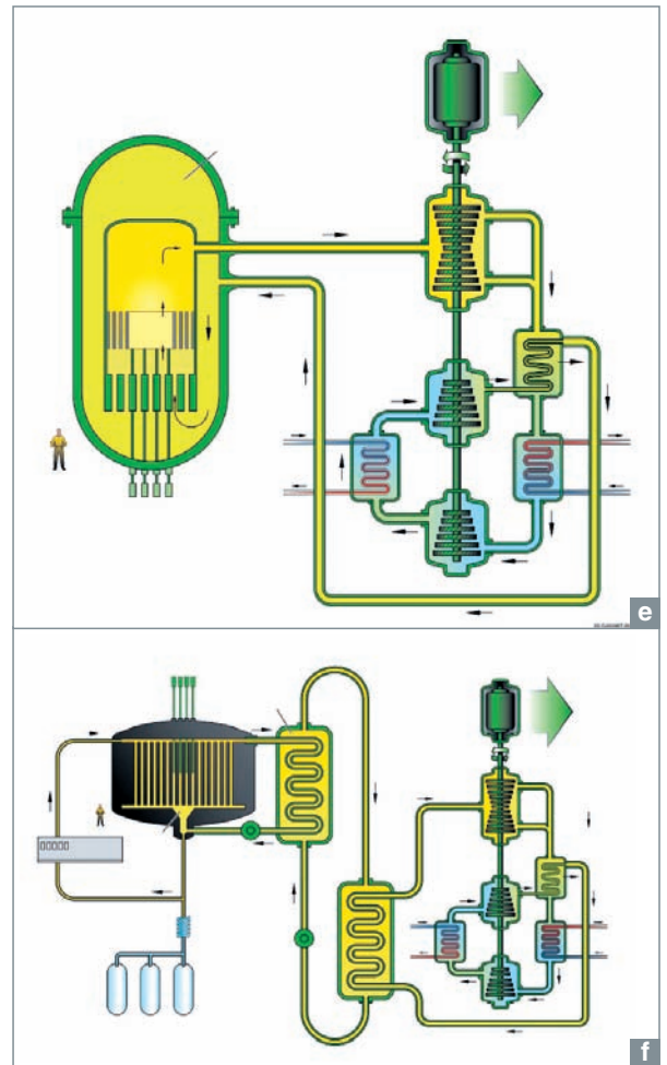
Fig. 3. Six systems selected by the Generation IV International Forum. Starting from the top left: a): SFR (sodium-cooled fast reactor); b): LFR (lead-cooled fast reactor); c): SCWR (supercritical water-cooled reactor); d): VHTR (very high temperature gas-cooled reactor); e): GFR (gas-cooled fast reactor); f): MSR (molten salt reactor). Two of the six systems chosen are gas-cooled.
