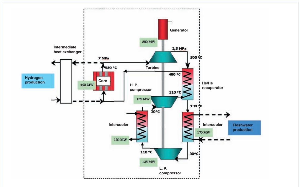
Fig. 59. Basic diagram of a VHTR using a direct helium cycle. The heat at 950 °C powers a high-performance turbomachine (high-efficiency electricity production) and a thermochemical cycle hydrogen
