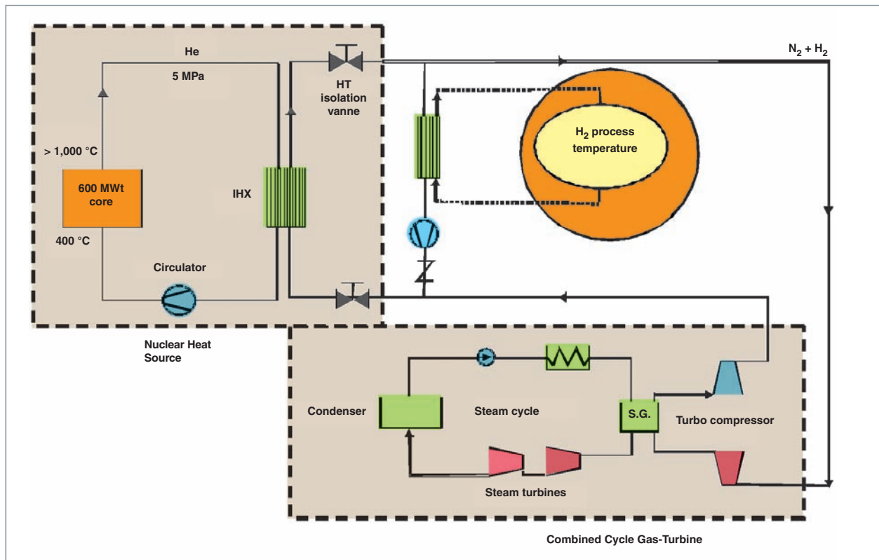
Fig. 26. Basic diagram of the ANTARES project. Due to the technological difficulties associated with the design and construction of a helium-cooled turbocharger, the ANTARES project is based on the implementation of an indirect cycle with an intermediate heat exchanger and a secondary circuit using nitrogen (whose properties are similar to those of air). This concept makes use of proven air turbine and compressor technologies. AREVA adds 20% helium to the nitrogen carrier gas so as to improve its exchange properties. This has the advantage of optimising the intermediate heat exchanger design without significantly affecting the conventional turbocharger technology implemented. The energy conversion system used in the ANTARES project implements a combined cycle consisting of a variation of the Brayton cycle with the turbine exhaust recuperator replaced by a steam generator powering a steam turbine. This combined cycle is similar to the one intended for combustion gas turbines, except that it uses a
