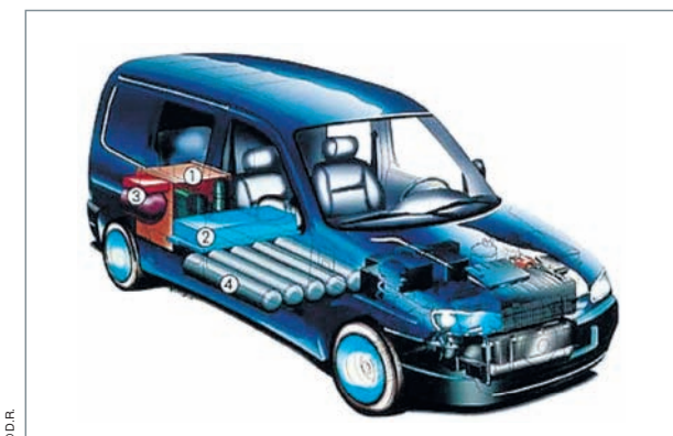
Fig. 2. Principle of a hydrogen-powered vehicle. Hydrogen can be used to power an internal combustion engine or a fuel cell.
