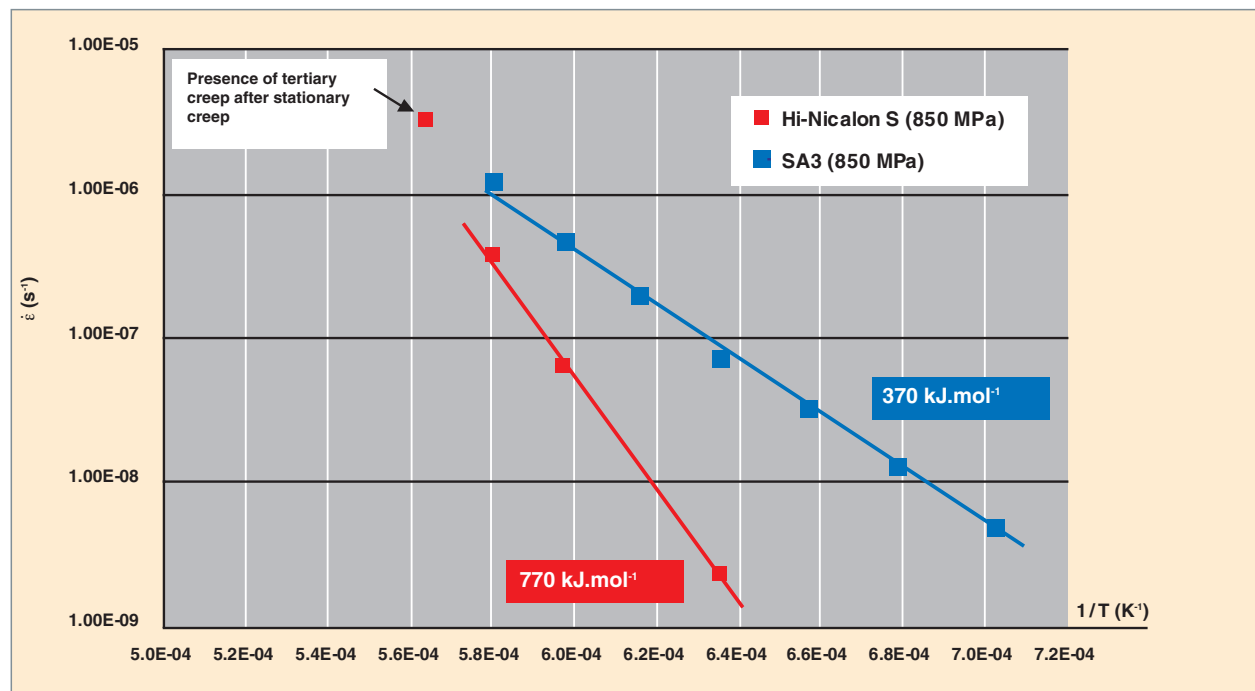
Fig. 66. Activation energy of the secondary thermal creep rate for two commercial SiC β fibers: Tyrano SA3 and Hi Nicalon S. For the SA3 fiber, the activation energy is close to the self-diffusion energy
