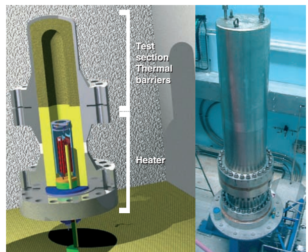
Fig. 85. The HETHIMO bench for testing thermal barriers.
