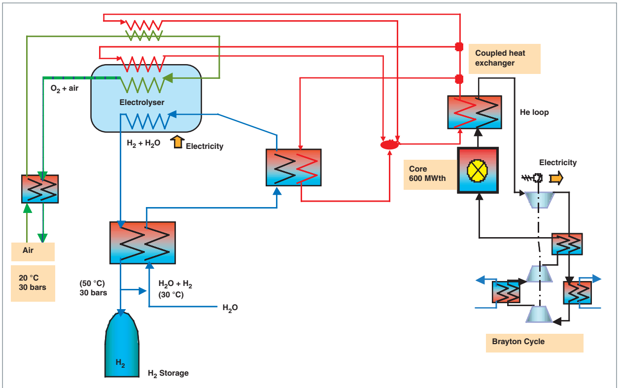
Fig. 81. Basic diagram of the coupling of a gas-cooled reactor with a high-temperature electrolyzer (modeled using the COPERNIC/CYCLOP program).
