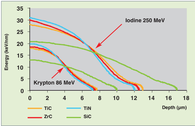
Fig. 117. Irradiation results at GANIL (Kr 86, 86 MeV, 5 \cdot 10^{15} ions/cm 2 ) and Vivitron (I 127, 250 MeV, 1 \cdot 10^{15} ions/cm 2 ): energy dissipation in ceramics of interest for GCR fuel.
