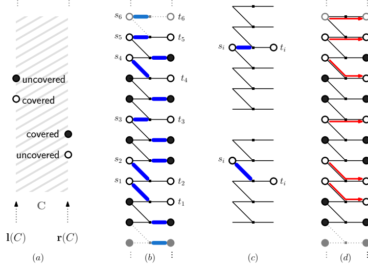
FIGURE 7. (a) The rules (19)-(20) that define the two Maya diagrams \mathbf{l}(C) and \mathbf{r}(C) . (b) An admissible dimer covering of the elementary rail yard graph L+ . White marbles are numbered as in the proof of Proposition 8. (c) If the left boundary vertex at ordinate s_i is covered by a horizontal (resp. diagonal) dimer, then the right boundary vertex at ordinate s_i (resp. s_i - 1 ) is necessarily uncovered. Therefore there is a white marble at this ordinate on the right boundary, and induction implies that it is the i -th white marble on the right boundary. This proves that s_i - t_i \in \{0, 1\} and that \sum_i (s_i - t_i) is equal to the number of diagonal dimers. Moreover, since dimers incident to the left boundary can be recovered from the knowledge of the sequences (s_i) and (t_i) , it is clear that there is at most one dimer configuration with given boundary states \mathbf{l} and \mathbf{r} , and that there is one if and only if (23) and (24) hold. (d) Condition (23) can be interpreted by saying that white marbles are “jumping downwards” by 0 or 1. The cases of the elementary graphs L- , R+ , and R- have similar interpretation, respectively with white marbles jumping upwards, black marbles jumping upwards, and black marbles jumping downwards, in all cases by 0 or 1.
