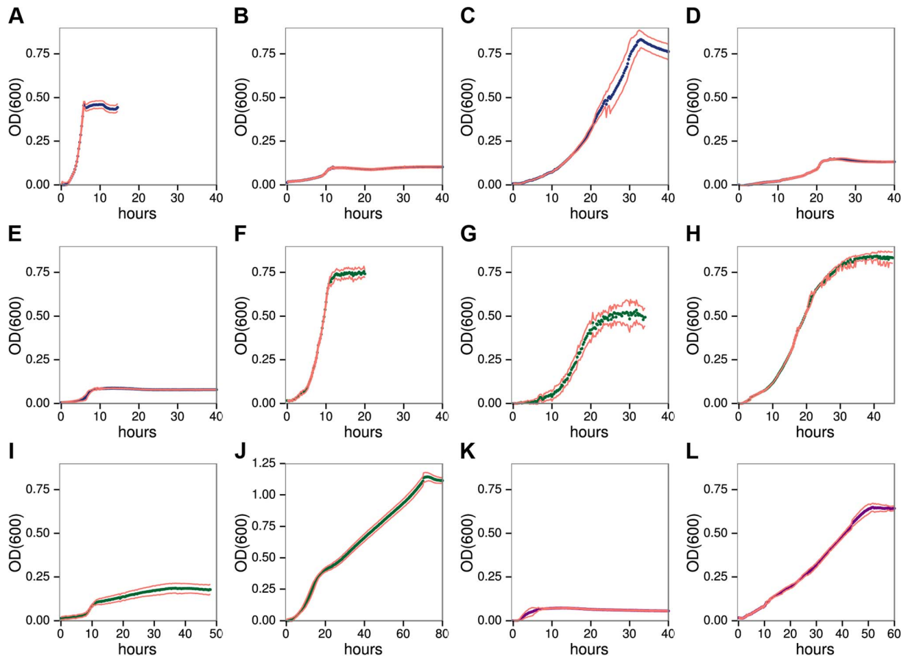
Figure 1. C. phytofermentans growth on pectic A-E , hemicellulosic F-J , and glucan K-L . Polysaccharides: homogalacturonan A , rhamnogalacturonan I B , galactan C , arabinan D , arabinogalactan II E , xylan F , arabinoxylan G , glucomannan H , galactomannan I , xyloglucan J , carboxymethylcellulose K , starch L . Growth was measured as OD 600 every 15 minutes. Each point is the mean of six cultures; red lines show one standard deviation.
