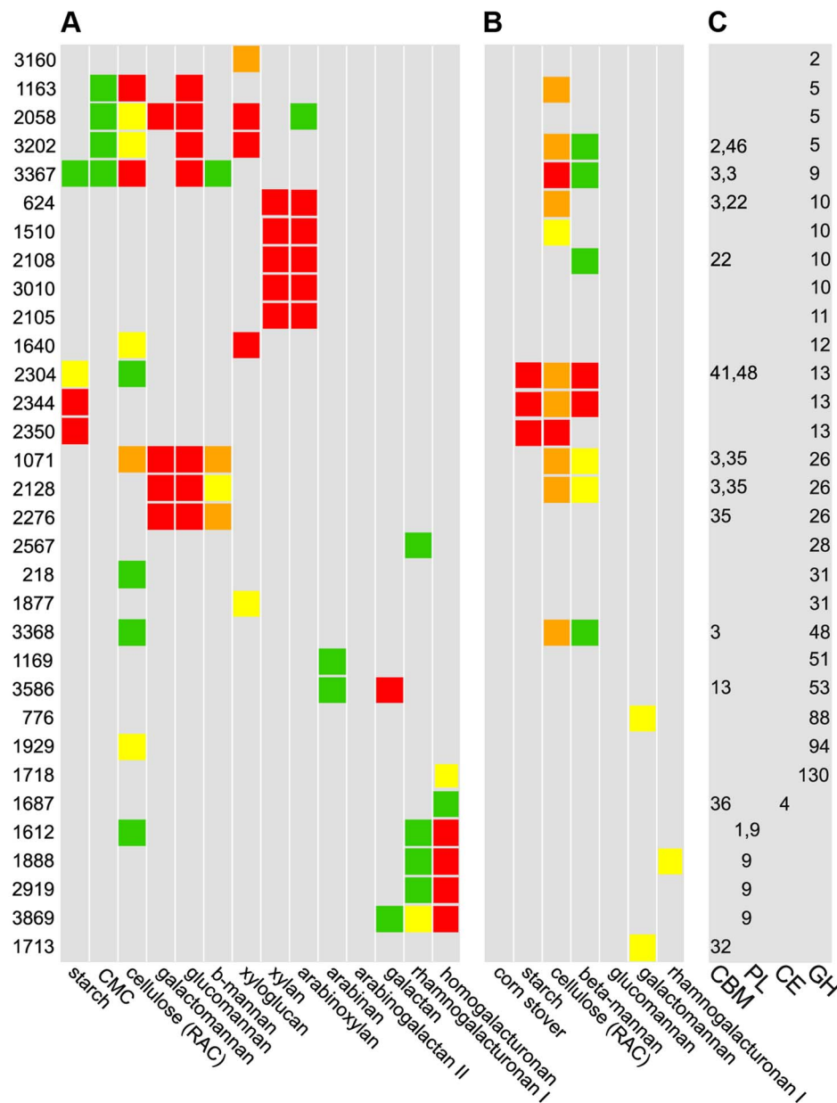
Figure 4. Cleavage A, binding B, and CAZy database classification C of purified enzymes. A Polysaccharide cleavage was quantified as nmol reducing sugar released per milligram enzyme per minute: >160 red, 80–160 orange, 40–80 yellow, 20–40 green, <20 gray. B Binding to insoluble polysaccharides was quantified as percentage enzyme bound to substrate: >30% red, 20–30% orange, 15–20% yellow, 10–15% green, <10% gray. C CAZy database classifications: glycoside hydrolases (GH), carbohydrate esterases (CE), polysaccharide lyases (PL), and carbohydrate binding domains (CBM). Among 56 purified CAZymes, only the 32 enzymes for which activities were found are shown. doi:10.1371/journal.pgen.1004773.g004
