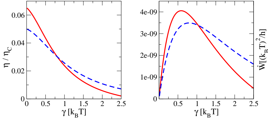
Figure 6. (Color online) Left panel: Efficiency \eta , normalized over the Carnot limit, as a function of the coupling energy \gamma . Right panel: Output power \dot{W} extracted from the system, as a function of the coupling energy \gamma . In both cases, the full red curves correspond to a three-terminal configuration with \gamma_2 = 0.5\gamma , while the dashed blue curve refer to the two-terminal case ( \gamma_2 = 0 ). Parameters: E_d - \mu = 2.0 k_B T , \Delta\mu_1 = -\Delta\mu_2 = -10^{-4} k_B T , \Delta T_1 = 10^{-3} T , and \Delta T_2 = 0 .
