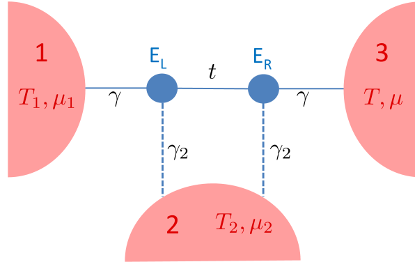
Figure 8. (Color online) Sketch of the double dot model used in the numerical simulations: two quantum dots with a single energy level are connected in series to three fermionic reservoirs 1, 2 and 3. The chemical potential and temperature of reservoir 3 are assumed as the reference values \mu and T . A two-terminal configuration is obtained in the case in which the coupling to reservoir 2 (equal for both the dots) vanishes ( \gamma_2 = 0 ).
