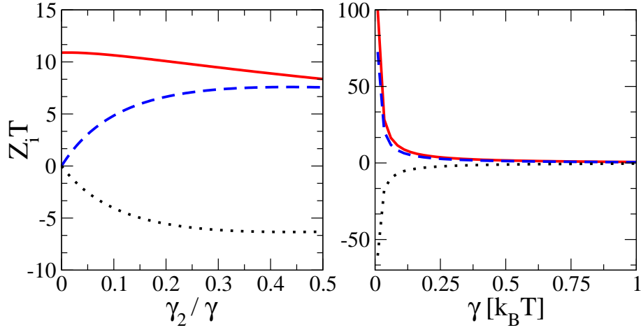
Figure 9. Various figures of merit Z_{11}^a T (dotted line), Z_{11}^b T (dashed line) and Z_{11}^c T (full line) as a function of the coupling to the bottom reservoir \gamma_2 (left panel), and as a function of the total coupling \gamma (right panel). Parameter values: E_L - \mu = -2 k_B T , E_R - \mu = -20 k_B T , \gamma = 0.1 k_B T (left panel) and \gamma_2 = 0.5 k_B T (right panel).
