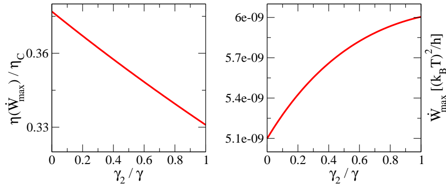
Figure 5. (Color online) Left panel: Efficiency at maximum power \eta(\dot{W}_{\max}) , normalized over the Carnot limit, as a function of the coupling to the reservoir 2. Right panel: Maximum output power \dot{W}_{\max} extracted from the system, as a function of the coupling to the reservoir 2. Parameters: \gamma = 0.1 k_B T , E_d - \mu = 2.0 k_B T , \Delta T_1 = 10^{-3} T , and \Delta T_2 = 0 .
