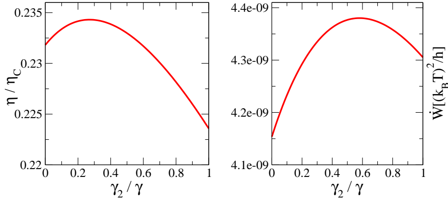
Figure 4. (Color online) Left panel: Efficiency \eta , normalized over the associated Carnot limit computed as in Sec. 3.1, as a function of the coupling to the reservoir 2. Note that as \gamma_2/\gamma is switched on, the efficiency increases until it reaches a maximum around \gamma_2 \sim 0.3\gamma , and then it decreases. Right panel: Output power \dot{W} extracted from the system, as a function of the coupling to the reservoir 2. Parameters: \gamma = 0.1 k_B T , E_d - \mu = 2.0 k_B T , \Delta\mu_1 = -\Delta\mu_2 = -5 \times 10^{-4} k_B T , \Delta T_1 = 10^{-3} T , and \Delta T_2 = 0 .
