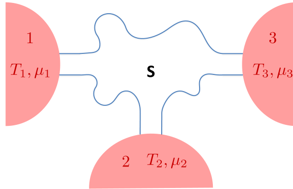
Figure 1. Three-terminal thermal machine. A scattering region is connected to 3 different fermionic reservoirs, each of these is able to exchange heat and particles with the system. Reservoir 3 is taken as the reference for measuring temperature and energy: T_3 \equiv T ; \mu_3 = \mu . The reservoirs 1 and 2 have small variations in temperature and chemical potential: (T_i, \mu_i) = (T + \Delta T_i, \mu + \Delta \mu_i) , i \in (1, 2) . With \mathbf{S} we denote a generic coherent scattering region.
