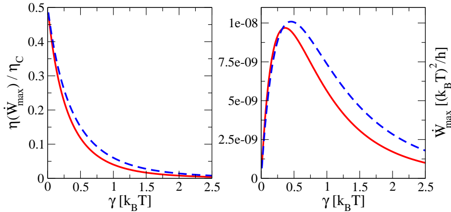
Figure 7. (Color online) Left panel: Efficiency at maximum power \eta(\dot{W}_{\max}) , normalized over the Carnot limit, as a function of the coupling energy \gamma . Right panel: Maximum output power \dot{W}_{\max} extracted from the system, as a function of the coupling energy \gamma . In both cases, the full red curves correspond to a three-terminal configuration with \gamma_2 = 0.5\gamma , while the dashed blue curves refer to the two-terminal case ( \gamma_2 = 0 ). Parameters: E_d - \mu = 2.0 k_B T , \Delta T_1 = 10^{-3} T , and \Delta T_2 = 0 .
