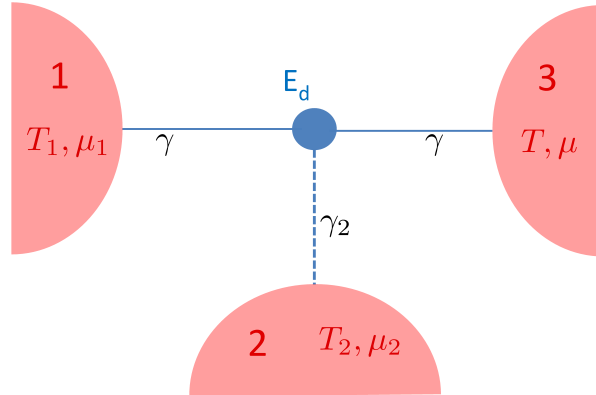
Figure 2. (Color online) Sketch of the single dot model used in the numerical simulations: a quantum dot with a single energy level E_d is connected to three fermionic reservoirs 1, 2, and 3. The chemical potential and temperature of the reservoir 3 are assumed as the reference values \mu and T . The constants \gamma and \gamma_2 represent the coupling between the system and the various reservoirs (see Appendix C.1 for details). A zero value of \gamma_2 corresponds to disconnecting the reservoir 2 from the system: in this regime the model describes a two-terminal device where reservoirs 1 and 3 are connected through the single dot.
