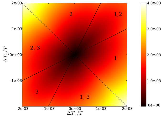
Figure 3. (Color online) Carnot efficiency \eta_C (density plot) of the three-terminal system depicted in Fig. 2, as a function of the gradients of temperature in reservoirs 1 and 2 (the chemical potentials \mu_1 and \mu_2 being chosen to guarantee maximum output power \dot{W} ). The coupling with the reservoirs have been set to have a symmetric configuration with respect to 1 and 2 (i.e. \gamma_2 = \gamma ). Note that \eta_C increases linearly along any radial direction defined by a relation \Delta T_2 = k\Delta T_1 , where k is a constant. In particular, the dashed lines corresponding to k = 0.5 , k = 2 and k = -1 separate different regimes discussed in Sec. 3.1. The numbers in each region identify the reservoirs from which the heat is absorbed. Parameter values: \gamma = 0.2k_B T , E_d - \mu = 2.0k_B T .
