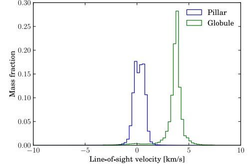
Fig. 15. Distribution of the gas mass as a function of the line-of-sight velocity for a pillar in the Mach-1 simulation and for a globule in the Mach-4 simulation (see Tremblin et al. 2012b, for the details of the numerical setup). Snapshots of the Mach 1 and Mach 4 simulations are in Fig. 11).
