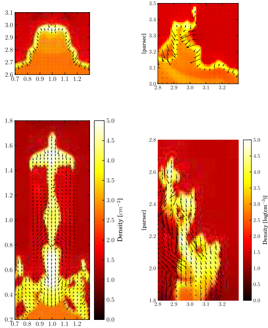
Fig. 13. Density cut of the formation of a pillar in an idealized simulation of a clump embedded in a homogeneous medium ( left : Tremblin et al. 2012a) and in a turbulent medium at Mach 1 ( right : Tremblin et al. 2012b). The black arrows represent the velocity field of the neutral gas. The compressed layer can be identified with the velocity field and the high density (around 10^4 \text{ cm}^{-3} in yellow). Top : the snapshots are taken when the pillar is forming, just before the compressed layer has collapsed in on itself. The high curvature of the compressed layer can be clearly identified in both cases. Bottom : after the shell has collapsed, the pillars are formed.
