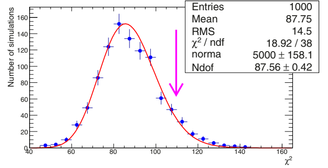
Fig. 24. Distribution of the \chi^2 obtained for 1000 simulations reproducing the 1D power spectrum measured by BOSS. The mean of the distribution is 87.8 and a fit of the distribution following a \chi^2 law defined in Eq. (17) gives a number of degrees of freedom equal to 87.6 \pm 0.4 .
