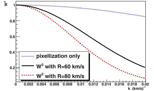
Fig. 10. Window function W^2(k, \bar{R}, \Delta v) , with \Delta v = 69 \text{ km s}^{-1} , reproducing the spectrum binning and the impact of the spectrograph resolution, for a resolution \bar{R} = 60 \text{ km s}^{-1} typical at \lambda > 5000 \text{ Å} and \bar{R} = 80 \text{ km s}^{-1} typical at \lambda < 4300 \text{ Å} . For comparison, we also show the contribution from only the pixellization (equivalent to \bar{R} = 0 ).
