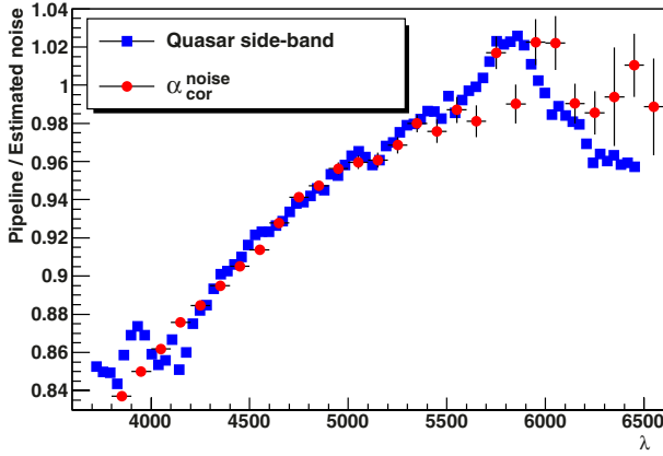
Fig. 1. Ratio of the pipeline noise estimate to the actual flux dispersion in the spectra. The blue squares denote this ratio as estimated from the quasar 1330 < \lambda_{\text{RF}} < 1380 \text{ \AA} and 1450 < \lambda_{\text{RF}} < 1500 \text{ \AA} sidebands. The red points indicate the correction from our procedure (Eq. (2)) as a function of mean forest wavelength.
