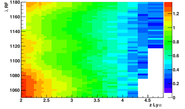
Fig. 7. Product of the quasar continuum C_q(\lambda, z_{\text{qso}}) by the mean transmitted flux fraction \bar{F}(z) as a function of rest-frame wavelength and Ly \alpha redshift. This 2D table is used to compute the normalized flux transmission fraction \delta(\lambda) .
