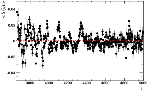
Fig. 9. Mean of \delta(\lambda) as a function of wavelength in Å. Systematic offsets from zero are seen at the 2% level due to imperfections in the spectrograph calibration.
