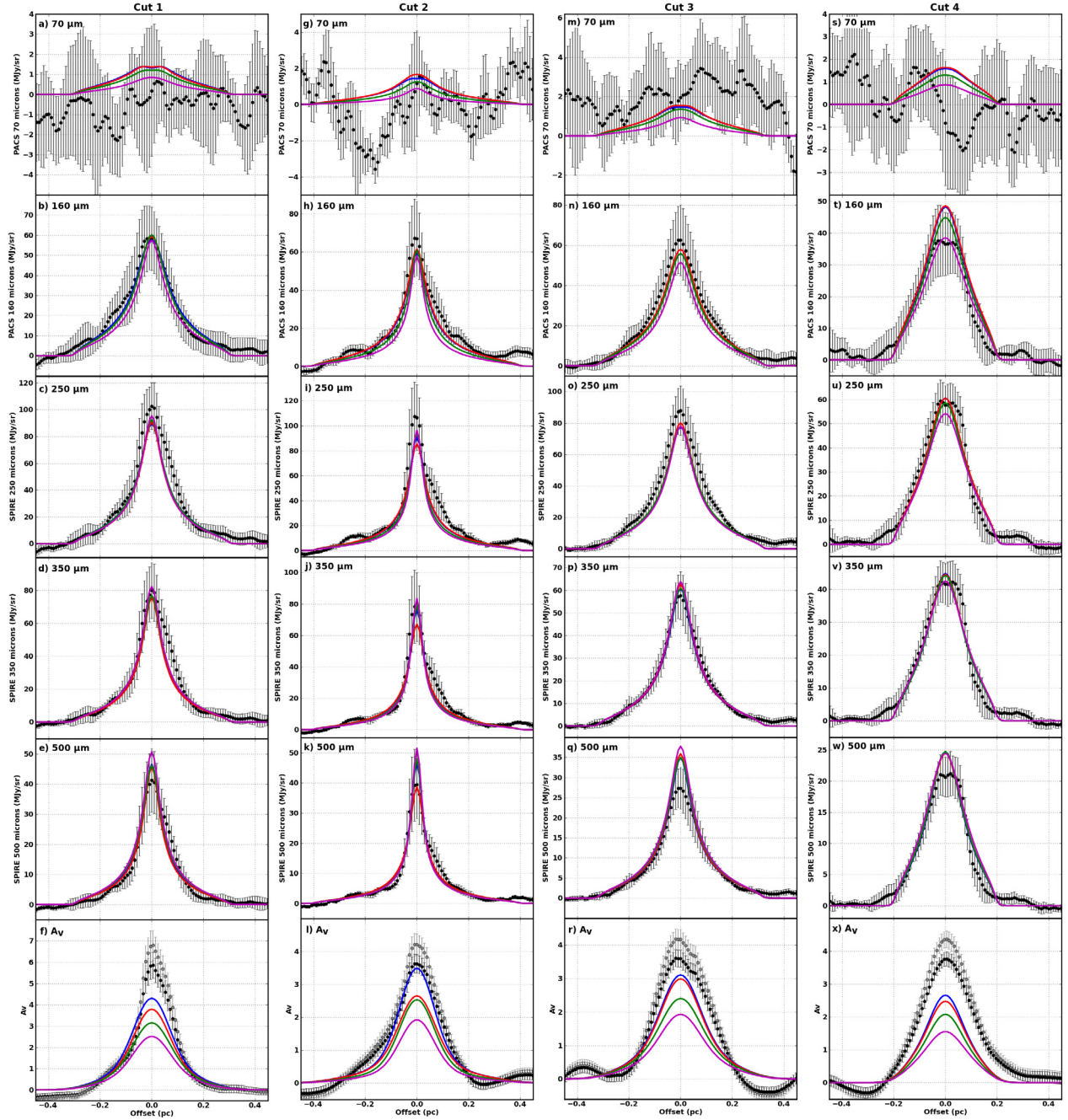
Fig. 6. The lines show the best fits with aggregates of the emission brightness profiles for the first cut at 70 \mu\text{m} a ); 160 \mu\text{m} b ); 250 \mu\text{m} c ); 350 \mu\text{m} d ); 500 \mu\text{m} e ); and the corresponding extinction profile f ). The grey dots show the extinction profile calculated from 2MASS with R_V = 3.1 and the black ones with R_V = 5.5 . The same are shown for the second cut g )– l ); the third cut m )– r ); and the fourth cut s )– x ). The blue lines are for compact aggregates, the red lines for aggregates with 10% of voids, the green lines with 25% of voids, and the magenta lines with 40% of voids.
