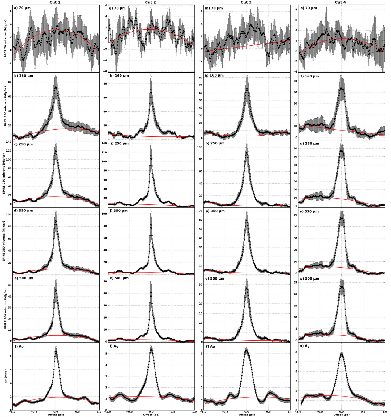
Fig. 4. Emission brightness profiles of the first cut (see Table 2) at 70 \mu\text{m} a ); 160 \mu\text{m} b ); 250 \mu\text{m} c ); 350 \mu\text{m} d ); and 500 \mu\text{m} e ); and extinction profile calculated from the 2MASS data with R_V = 3.1 f ). The same for the second cut g )– l ); the third cut m )– r ); and the fourth cut s )– x ). The red lines show the second order polynomials fitted to remove the relatively diffuse envelope from the densest filament.
