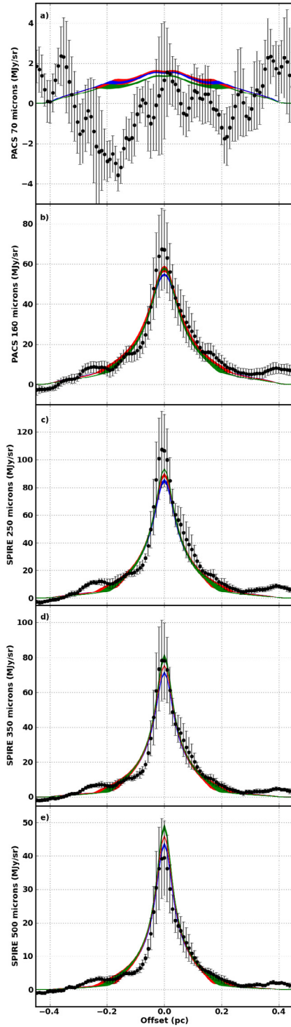
Fig. 9. Brightness profiles of the second cut at 70, 160, 250, 350, and 500 \mu\text{m} (panels a ); b ); c ); d ); and e ) respectively). The blue areas are the best-fitting models for compact aggregates and n_T = 875 \pm 125 \text{ H/cm}^3 , the red ones for porous aggregates with 10% of voids and n_T = 750 \pm 250 \text{ H/cm}^3 , and the green ones for porous aggregates with 25% of voids and n_T = 625 \pm 125 \text{ H/cm}^3 .
