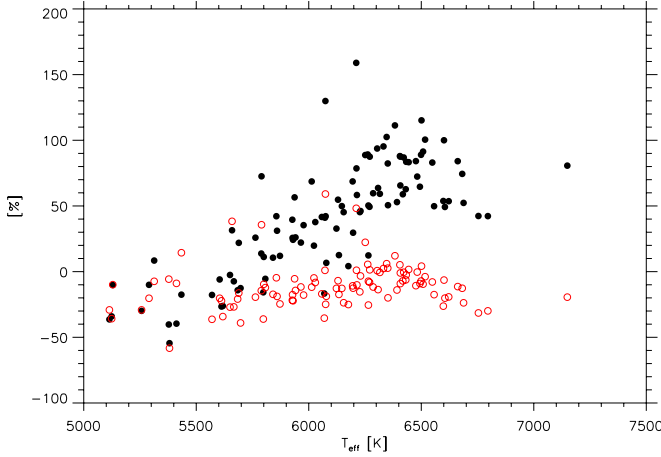
Fig. 6. Relative differences (in %) between the theoretical \sigma and the measured ones as a function of T_{\text{eff}} . The black filled circles correspond to the relative difference D_\sigma = (\sigma_{\text{theo}}/\sigma_{\text{m}}) z_3 - 1 and the red open circles to the relative difference D'_\sigma = (\sigma_{\text{theo}}/\sigma_{\text{m}}) c_3 - 1 , where z_3 (Eq. (19)) is the new theoretical scaling relation, c_3 (Eq. (20)) is the classical one, and \sigma_{\text{m}} the measurements (see details in Appendix A.2).
