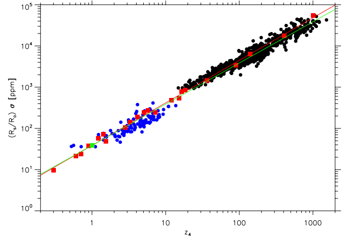
Fig. B.1. \tilde{\sigma} \equiv (R_s/R_\odot) \sigma as a function the quantity z_4 given by Eq. (B.2). The symbols have the same meaning as in Fig. 1. The green line corresponds to a linear scaling with z_4 and the red one to a power law of the form z_4^p where the slope p = 1.03 is obtained by fitting the individual theoretical values of \tilde{\sigma} (red squares).
