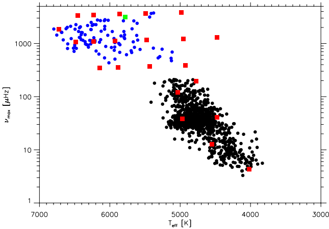
Fig. 1. \nu_{\text{max}} as a function of T_{\text{eff}} . The filled red squares correspond to the location of the 3D hydrodynamical models in the plan \nu_{\text{max}} - T_{\text{eff}} (see also Table 1), the filled blue circles to the Kepler sub-giant and MS targets, and the black ones to the Kepler red giants (see Sect. 5). The filled green square shows the position of our 3D solar model (the last model in Table 1).
