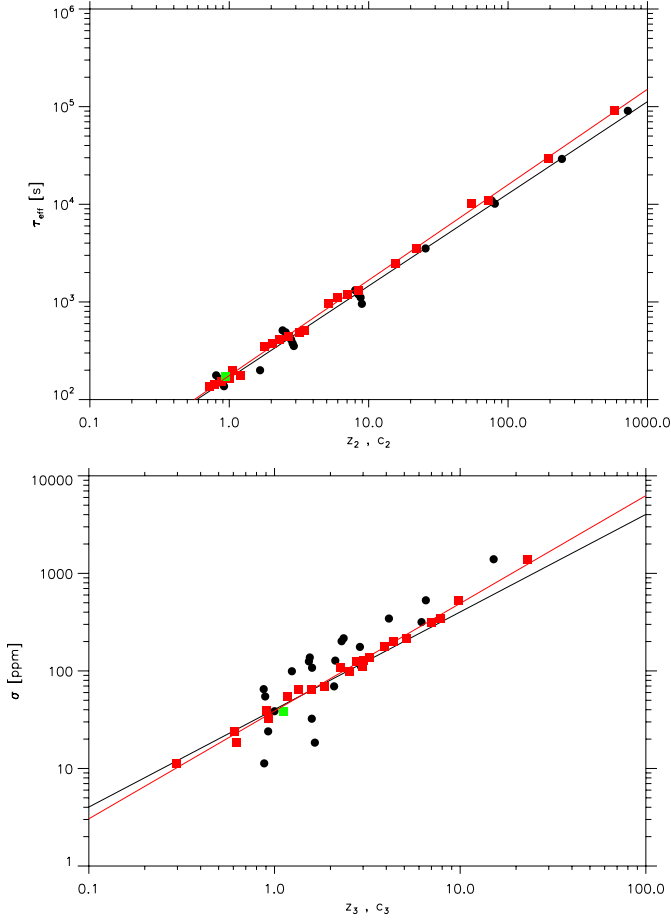
Fig. 3. Top: theoretical values of \tau_{\text{eff}} as a function of the quantity z_2 (red squares) given by Eq. (18) and as a function of the classical scaling c_2 \equiv (\nu_{\text{ref}}/\nu_{\text{max}}) (filled black circles). The symbols correspond to the individual theoretical values obtained with our grid of 3D models. The red curve corresponds to a power law of the form z_2^p where the slope p = 0.98 is obtained by fitting the red squares, while the black line is a power law of the form c_2^n where the slope n = 0.94 is obtained by fitting the black circles. Bottom: theoretical values \sigma as a function of the quantity z_3 given by Eq. (19) and as a function of the classical scaling c_3 (Eq. (20)). The symbols correspond to the individual theoretical values obtained with our grid of 3D models. The red curve is a power law of the form z_3^p where the slope p = 1.10 is obtained by fitting the red squares, while the black line is a linear scaling in c_3 .
