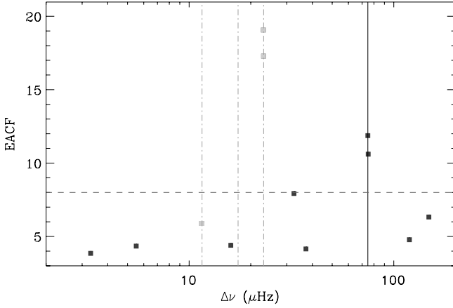
Fig. 4. Automatic determination of the large separation. Dark squares indicate the values of EACF tested in 13 frequency ranges between 2 and 220 \mu\text{Hz} . Gray values are artifacts caused by the CoRoT low Earth orbit and must be excluded. The horizontal dashed line indicates the threshold level for a detection at the 1% rejection level. The vertical dark gray line indicates the observed signature at \Delta\nu \approx 75 \mu\text{Hz} , and the dash-dotted lines the spurious signatures of the daily aliases (11.6 and 23.2 \mu\text{Hz} ).
