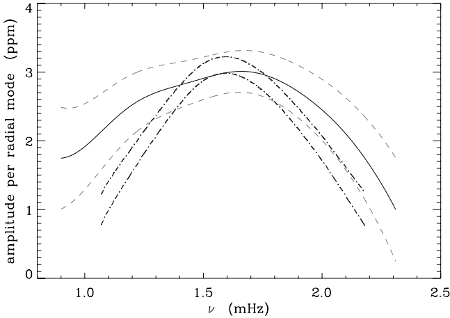
Fig. 6. Amplitude per radial mode determined according to Michel et al. (2009) for HD 175272 (solid line + dashed lines indicating the \pm 1 - \sigma uncertainty) and for the reference HD 181420 (mixed lines indicating the uncertainty). Error bars are principally due to the uncertainty in the power density of the background.
