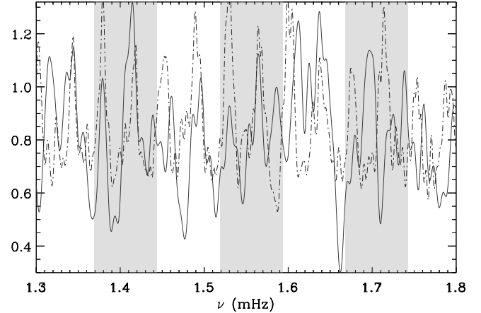
Fig. 5. Smoothed density spectrum of HD 175272 (Gaussian filter of width 5 \mu\text{Hz} ). Gray and white domains indicate frequency ranges with a width equal to the mean large separation. The dot-dashed line gives the spectrum of HD 181420, with frequencies multiplied by a factor 0.996, also smoothed and corrected for the difference between the white-noise contributions.
