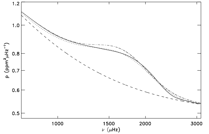
Fig. 3. Smoothed power density spectrum (with an apodized 300\text{-}\mu\text{Hz} FWHM window) in log-scale axes. The dashed line represents the contributions of the granulation signal and of the photon noise. The dotted line is a Gaussian fit of the excess power envelope. The mixed line is the smoothed spectrum of HD 181420, with the same treatment and an offset accounting for the different photon-noise levels.
