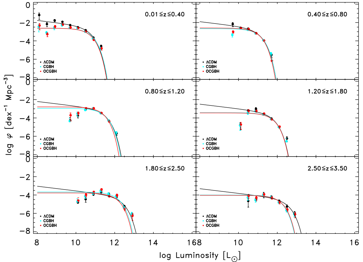
Fig. 4. As Fig. 3 for the rest-frame 160 \mu\text{m} 1/V_{\text{max}} luminosity functions. Here the effective wavelength is 90 \mu\text{m} .
