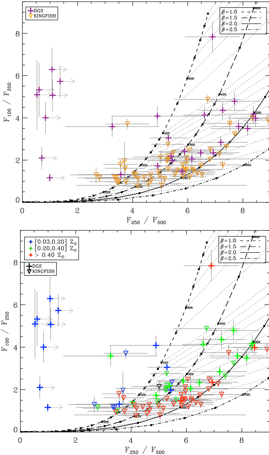
Fig. 10. Colour–colour diagram: PACS/SPIRE diagram: F_{100}/F_{250} versus F_{250}/F_{500} . The colour and symbol choices are the same as in Fig. 9 for both figures. Note that the most metal-poor galaxies (from 0.03 to 0.20 Z_{\odot} ) are very faint and even not detected anymore at long wavelengths. We were only able to derive upper limits beyond 160 \mu\text{m} for these galaxies and, thus, some galaxies do not appear on this diagram anymore.
