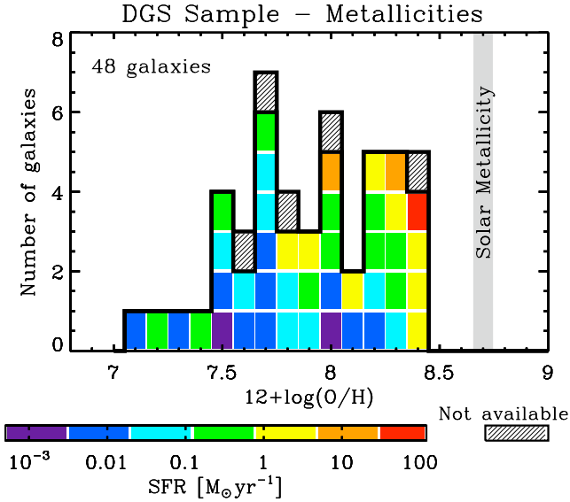
Fig. 1. Metallicity distribution of the DGS sample from 12 + \log(\text{O}/\text{H}) = 7.14 to 8.43 . Solar metallicity is indicated here as a guide to the eye. The pre- Herschel star formation rate (SFR) distribution is also indicated by the colour code. They have been converted from L_{\text{TIR}} ( Spitzer ) with the Kennicutt (1998) law, and are given in Madden et al. (2013). When no IR data was available, \text{H}\alpha or \text{H}\beta emission lines were used and converted to SFR (Kennicutt 1998). The dashed cells indicate that none of these data were available for the galaxy. The most actively star-forming galaxy (in red) corresponds to the starburst luminous infrared galaxy (LIRG) Haro 11.
