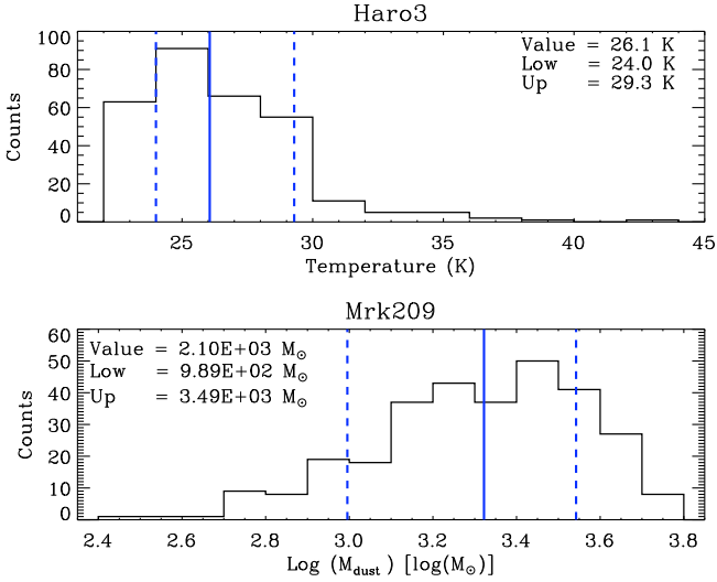
Fig. 12. Examples of the obtained parameter distributions for the 300 Monte-Carlo iterations for the modified blackbody fits: (top) distribution of temperature, T , for Haro 3, (bottom) distribution of dust mass, M_{\text{dust}} , for Mrk 209 with the 70\ \mu\text{m} point included in the fit. The plain blue line notes the value of the parameter and the dashed blue lines note the 66.67% confidence level for the parameters.
