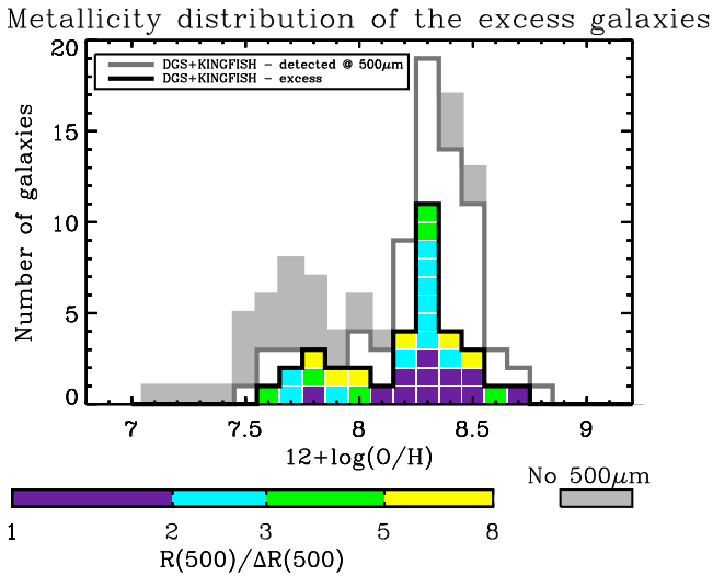
Fig. 17. Metallicity distribution for the excess galaxies in black. The colours mark the presence of an excess at 500\ \mu\text{m} and code the intensity of this excess: R(500)/\Delta R(500) . The metallicity distribution for the DGS & KINGFISH galaxies detected at 500\ \mu\text{m} is outlined in grey. The grey cells mark all of the galaxies for which no detection is available at 500\ \mu\text{m} .
