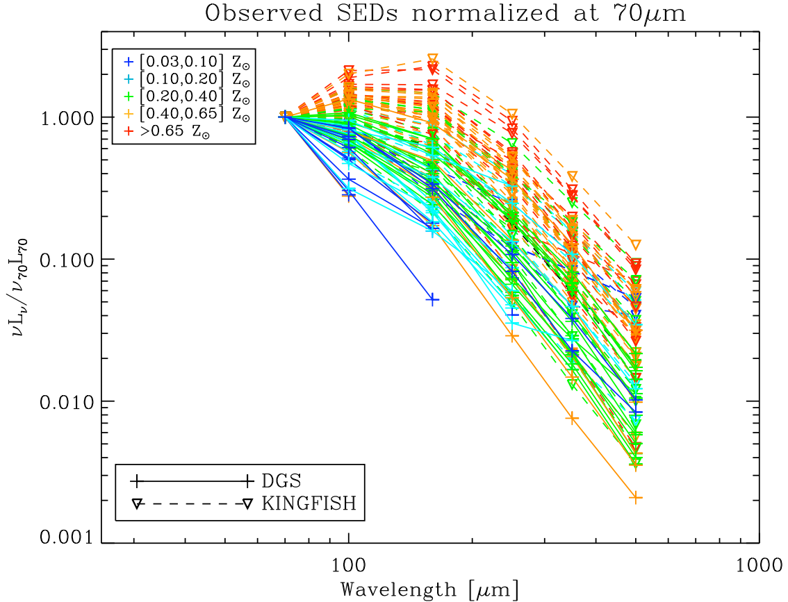
Fig. 8. Total Herschel observed SEDs for both DGS and KINGFISH samples, normalized at 70\ \mu\text{m} . The colours delineate the different metallicity bins, and the lines and symbols differentiate DGS (plain lines and crosses) and KINGFISH galaxies (dashed lines and downward triangles).
