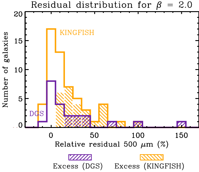
Fig. 16. Relative residual distribution at 500\ \mu\text{m} for modified blackbody fits with a fixed \beta_{\text{theo}} of 2.0 for DGS (purple) and KINGFISH (orange) samples. Galaxies for which the residual at 500\ \mu\text{m} is greater than the corresponding error bar ( R(500) > \Delta R(500) ) have been marked by hashed cells.
