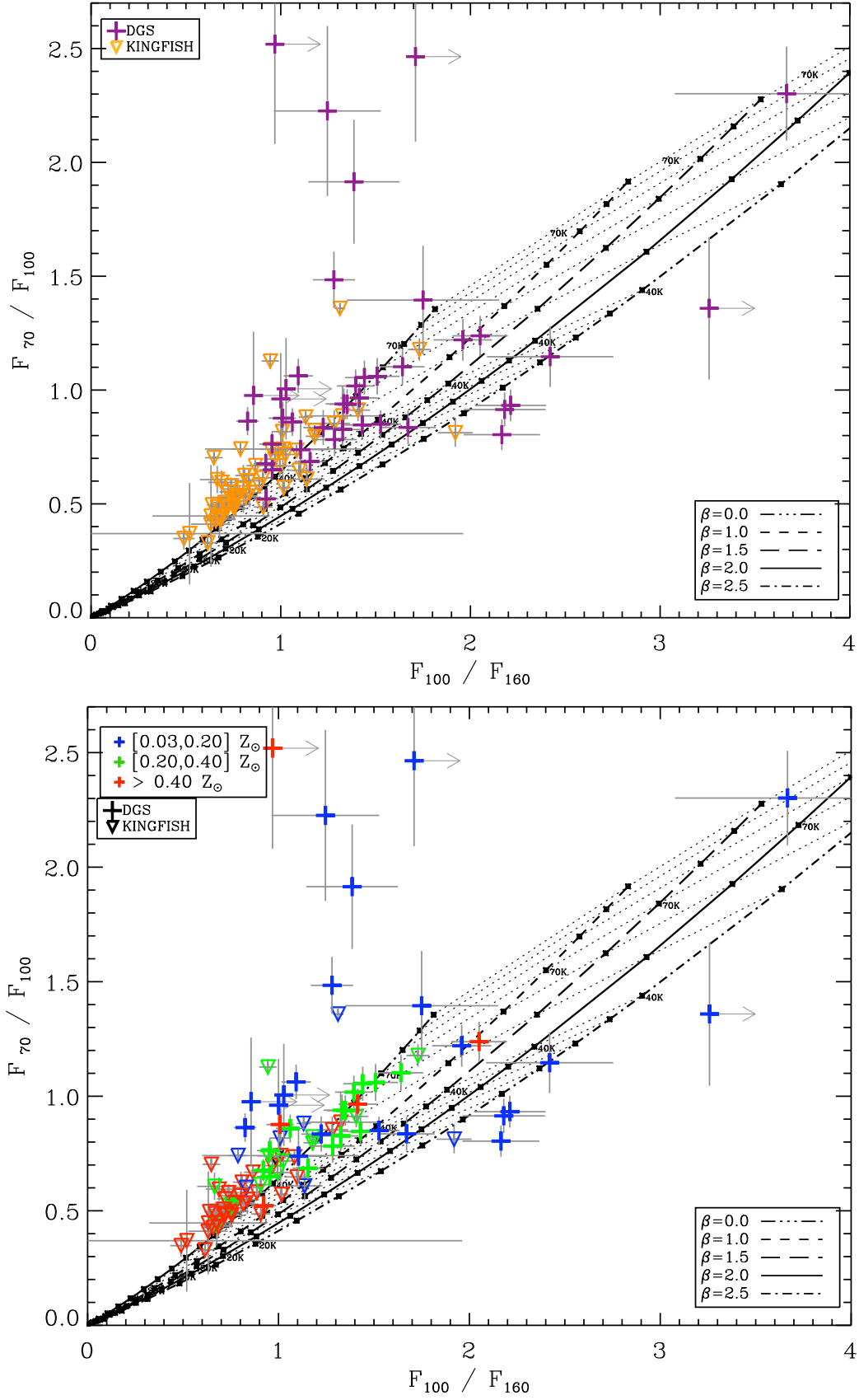
Fig. 9. Colour–colour diagram: PACS/PACS diagram: F_{70}/F_{100} versus F_{100}/F_{160} . Top: the colour and symbol code differentiates DGS (purple crosses) and KINGFISH galaxies (orange downward triangles). Bottom: the colour code delineates the different metallicity bins this time. Crosses and downward triangles are still representing DGS and KINGFISH galaxies, respectively. For both plots, the curves give theoretical Herschel flux ratios for simulated modified black bodies for \beta_{\text{theo}} = 0.0 to 2.5 and T from 0 to 40 K in 2 K bins and from 40 to 100 K in 10 K bins, as black dots, increasing in T from left to right. Lines of constant T are indicated as dotted lines, and a few temperatures have been marked on the plots.
