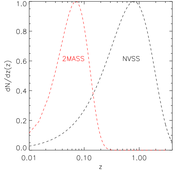
Fig. 3. Redshift distributions for 2MASS (see Afshordi et al. 2004; Rassat et al. 2007; Dupe et al. 2011) and NVSS (from Ho et al. 2008).
