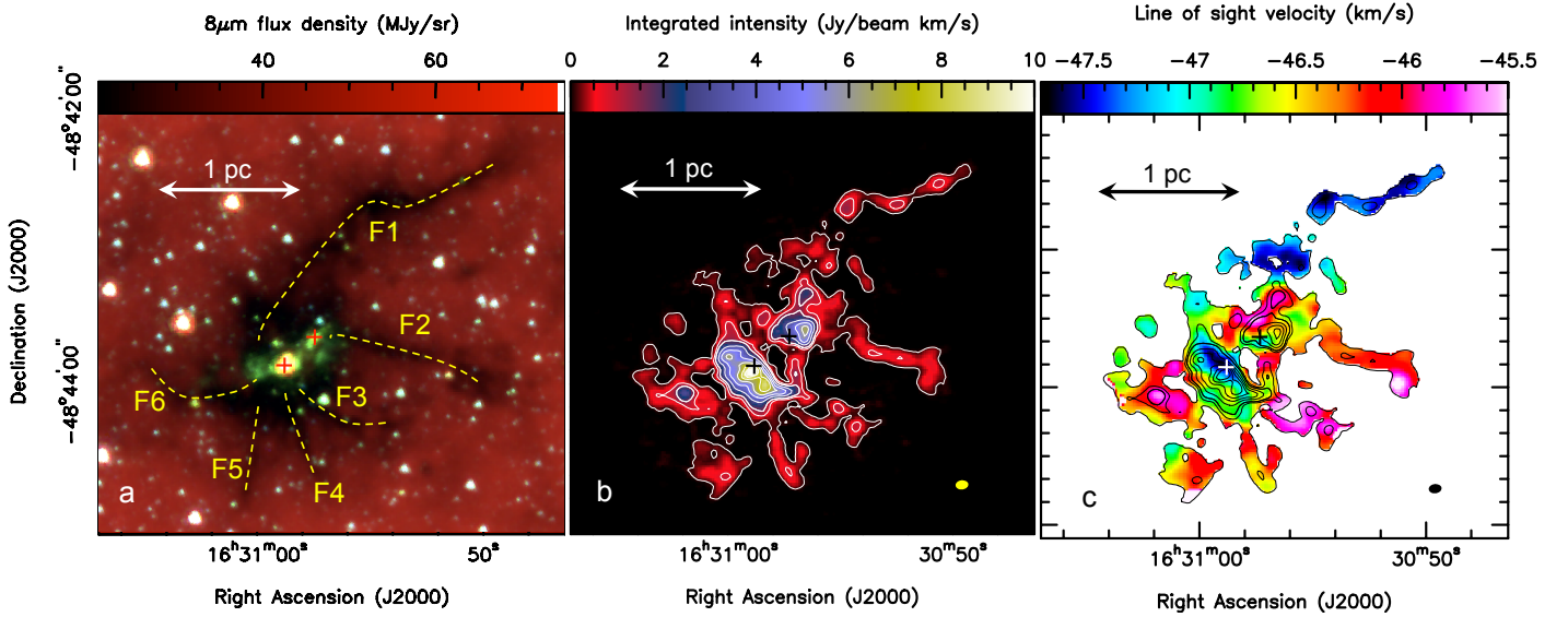
Fig. 4. a) Same as in Fig. 1a; b) ALMA-only image of the \text{N}_2\text{H}^+(1-0) integrated intensity over the 7 hyperfine structure components. The rms noise on the resulting map is \sim 6 mJy/beam km s ^{-1} . The contours go from 0.1 to 1.5 in steps of 0.7 Jy/beam km s ^{-1} and 1.5 to 9 in steps of 1.5 Jy/beam km s ^{-1} . The crosses mark the positions of the two dense cores. The ALMA beam is represented as a yellow elliptical symbol in the bottom-right corner of the image. We can see the excellent match between the Spitzer dust extinction of the filaments and the \text{N}_2\text{H}^+(1-0) emission; c) ALMA \text{N}_2\text{H}^+(1-0) velocity field using the first order moment map. The crosses mark the positions of the cores and the contours are the same as in the b) panel.
