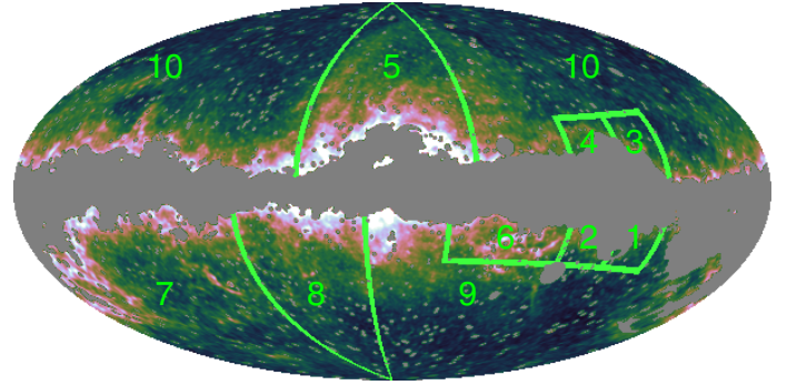
Fig. 1. Regions used in our multi-region RG template fits (see Sect. 3.1 and Table 1).
