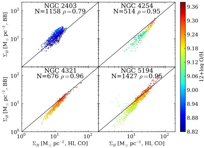
Fig. B.1. Total gas surface density derived from a modified black-body fit (Eq. (B.1)) of the FIR data from 70\ \mu\text{m} to 350\ \mu\text{m} versus the total gas surface density derived from the combination of HI and CO observations. The colour of each dot indicates the metallicity indicated by the scale on the right. The black lines show the 1-to-1 relation between these quantities.
