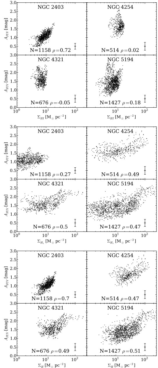
Fig. 3. Attenuation in the FUV band versus the atomic ( top ), molecular ( middle ), and total ( bottom ) gas mass surface density in units of M_\odot \text{pc}^{-2} for individual regions in galaxies (sample A). Each data point corresponds to a single pixel which has been detected at a 3\text{-}\sigma level from the FUV to the FIR. No selection has been applied on CO and HI data. Data points with a poor fit ( \chi^2 \geq 2 ) have also been removed. At the bottom of each panel we display the number of selected pixels N and the Spearman correlation coefficient \rho . Finally, the median uncertainty on A_{\text{FUV}} computed by CIGALE is indicated in the bottom-right corner .
