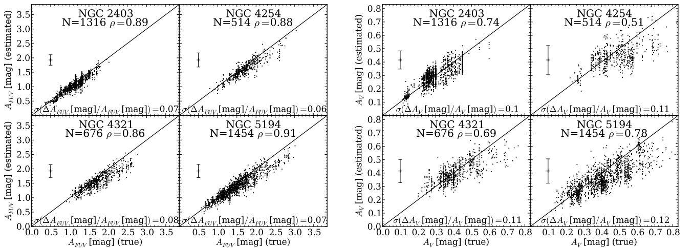
Fig. 2. Attenuation derived from the analysis of the probability distribution function performed with CIGALE versus the true value for artificial regions in galaxies, in order to test the accuracy of the modelling. In each quadrant we indicate the number of data points N , the Spearman correlation coefficient \rho at the top, and the scatter of the relative difference in the attenuation at the bottom. The solid black line indicates the 1-to-1 relation. The error bar on the left indicates the median uncertainty as computed from the analysis of the probability distribution function. For consistency with the analysis carried out later in this paper, we have only selected datapoints with a good best fit ( \chi^2 < 2 ). The left panel describes the FUV-band attenuation whereas the right one describes the V-band attenuation.
