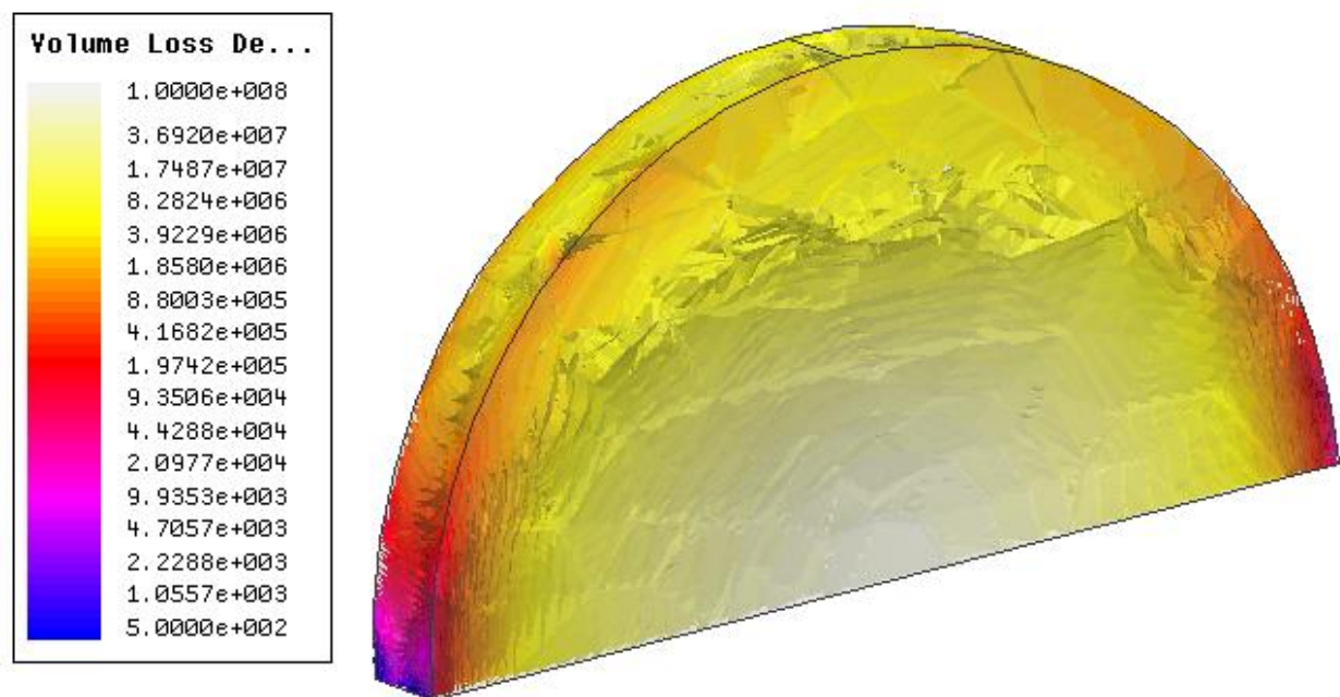
Figure 7. Dielectric losses distribution in \text{W/m}^3 in the ceramic for 500 kW input on matched load. The volume integrated loss in the ceramic is of the order of 550 W.
