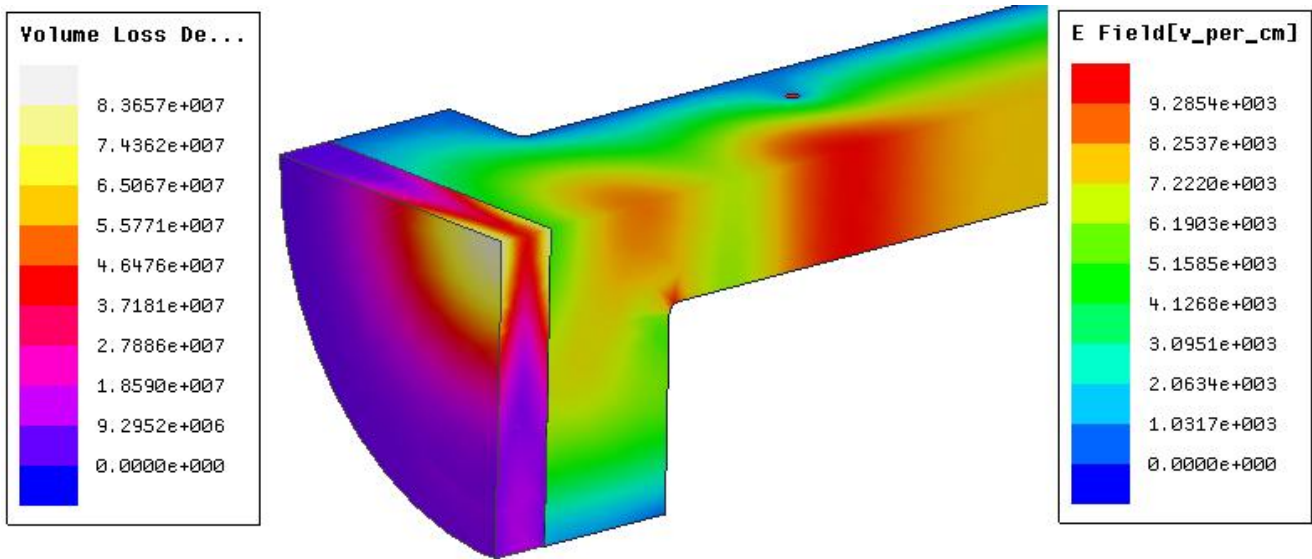
Figure 2. Volume loss density in the ¼ ceramic (left scale in W/m³) and electric field norm (right scale in V/cm) for 500 kW input on matched load.
