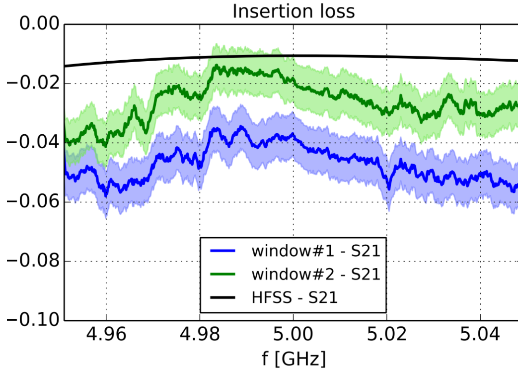
FIGURE 11. Insertion loss [dB] for both windows. RF modelling prediction(plain black) from HFSS. Bold line represent the averaged values and shaded areas the minimum and maximum of the measurement noise.
