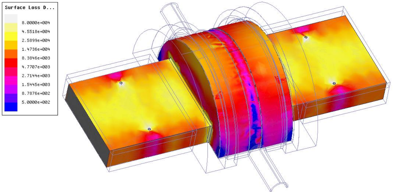
Figure 6. RF Resistive Heat Flux for 500 kW input power in \text{W/m}^2 . The surface integrated loss on the conductor is of the order of 720 W with a pessimistic copper conductivity of \sigma=44 \text{ MS/m} .
