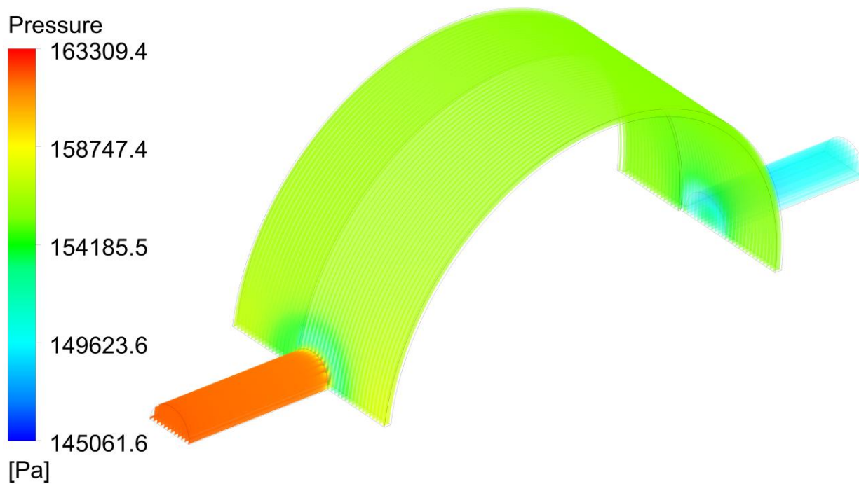
Figure 5. Water pressure in the skirt around the ceramic. Inlet is located at the left of the picture.
