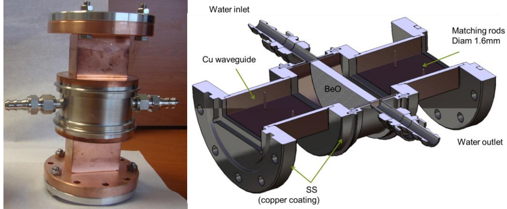
FIGURE 2). Left: picture of one window. Right: CAD cut-view of the window.
