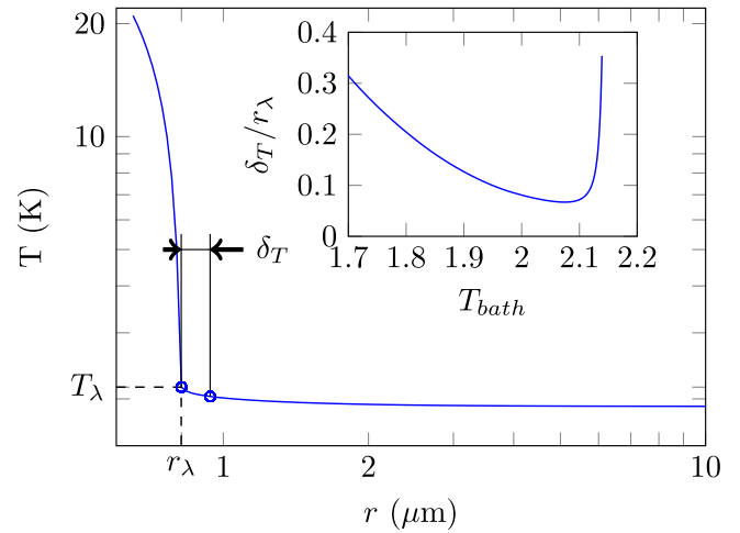
FIG. 4. Typical radial temperature profile around the wire, computed for T_{bath} = 1.91 \text{ K} . Inset: Thermal boundary layer in He II \delta_T normalized by r_\lambda , the radius of He I region.
