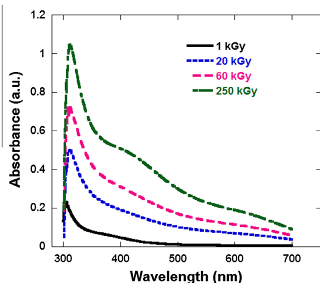
Fig. 9. Absorption spectra of ion-exchanged silicate glass (10% AgNO 3 ) and gamma irradiated at doses 1; 20; 60 and 250 kGy.
