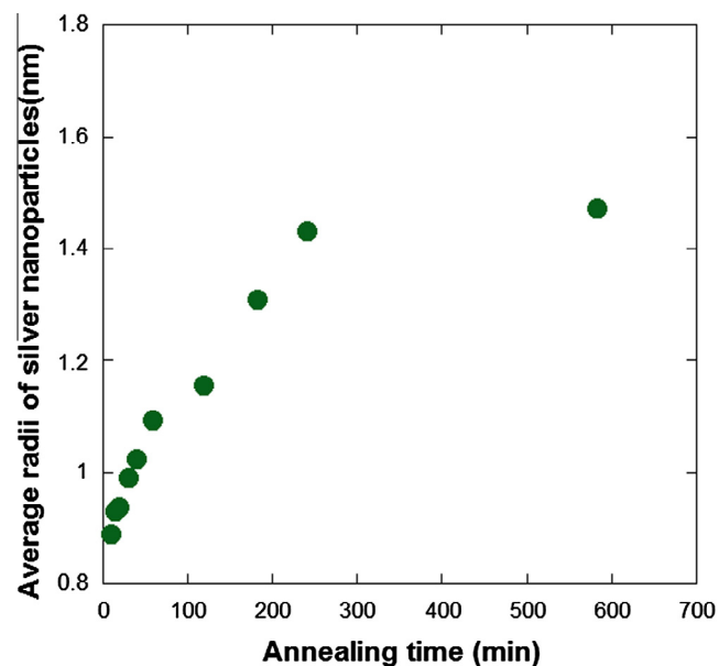
Fig. 7. Growth of silver aggregates as a function of annealed time (550 °C) in a glass exchanged to 5% AgNO 3 and irradiated by \gamma radiation to 250 kGy.
