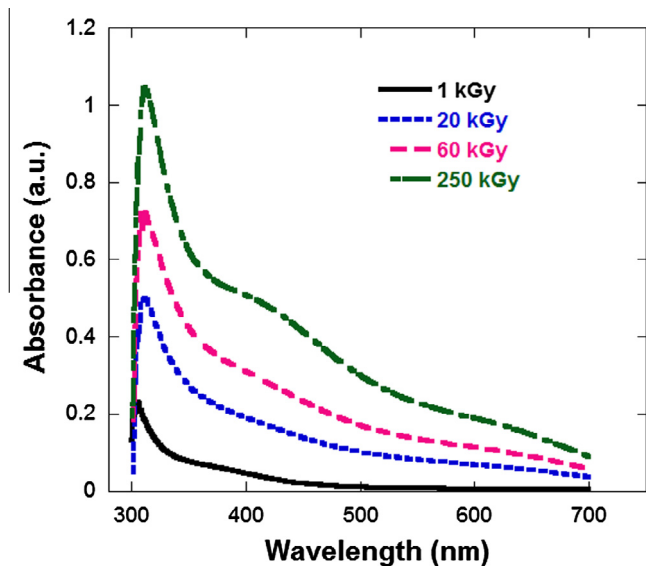
Fig. 9. Absorption spectra of ion-exchanged silicate glass (10% \text{AgNO}_3 ) and gamma irradiated at doses 1; 20; 60 and 250 kGy.
