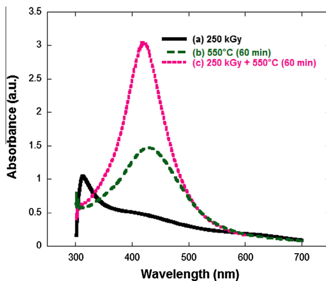
Fig. 4. Absorption spectra of ion-exchanged silicate glass, under the following conditions: (a) irradiated with \gamma rays at 250 kGy; (b) annealed at 550 °C for 60 min; and (c) irradiated at 250 kGy and annealed at 550 °C for 60 min.
