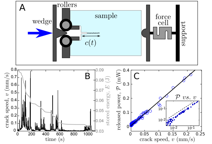
FIG. 1. A: Sketch of the Wedge-Splitting test. B: Zoomed view of the crack tip speed v(t) (black) and stored mechanical energy E(t) (gray) as a function of time in a typical fracture experiment (Here, V_{wedge} = 16 nm/s). C: Instantaneous power release \mathcal{P} = -dE/dt as a function of v(t) for all t . The axes are linear in the main panel, and logarithmic in the inset. In both panels, straight lines indicate proportionality. The proportionality constant \Gamma = 100 \pm 10 J/m 2 gives the material's fracture energy. In both panels B and C, the coarse-graining time is \delta t = 0.2 s
