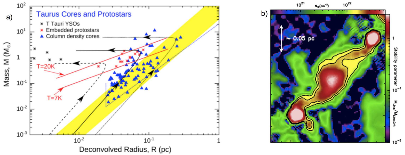
Fig. 8.— (a) Mass versus size diagram for the cores identified with Herschel in the Taurus S1/S2 region (J. Kirk et al. , 2013). The two red solid lines mark the loci of critically self-gravitating isothermal Bonnor-Ebert spheres at T = 7 K and T = 20 K, respectively, while the yellow band shows the region of the mass-size plane where low-density CO clumps are observed to lie (cf. Elmegreen and Falgarone, 1996). The blue dotted curve indicates both the mass sensitivity and the resolution limit of the Kirk et al. (2013) study. Model evolutionary tracks from Simpson et al. (2011) are superposed as black lines (dashed, solid, and dotted for ambient pressures P_{\text{ext}}/k_B = 10^6 \text{ K cm}^{-3} , 10^5 \text{ K cm}^{-3} , and 10^4 \text{ K cm}^{-3} , respectively), in which starless cores (blue triangles) first grow in mass by accretion of background material before becoming gravitationally unstable and collapsing to form protostars (red stars) and T Tauri stars (black stars). (b) Blow-up Herschel column density map of a small portion of the Taurus B211/B213 filament (cf. Fig. 2a) showing two protostellar cores on either side of a starless core (Palmeirim et al. , in prep.). The contrast of filamentary structures has been enhanced using a curvelet transform (see Starck et al. , 2003). Note the bridges of material connecting the cores along the B211/B213 filament, suggesting that the central starless core may still be growing in mass through filamentary accretion, a mechanism seen in some numerical simulations (cf. Balsara et al. , 2001 and § 5).
