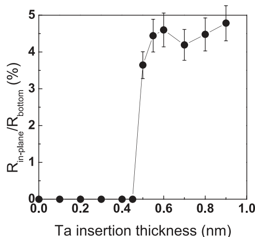
FIG. 3. Relative Hall contribution of the in-plane component of the bottom electrode as a function of the Ta insertion thickness.
