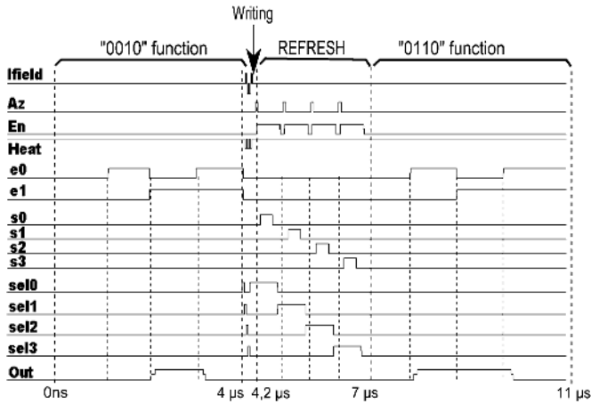
Fig. 9. Dynamic reconfiguration.
