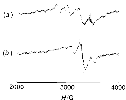
Fig. 3 EPR spectra of an LB film of \text{ZnP}(\text{N}^+\text{C}_{22})_4/\text{CuPcTS}^{4-} heterodimers alternated with \omega -tricosenoic acid (680 layers). (a) Magnetic field perpendicular to the substrate plane, g = 2.1490 ; (b) magnetic field parallel to the substrate plane, g = 2.052 . T = 300 K, \nu = 9.4698 GHz
