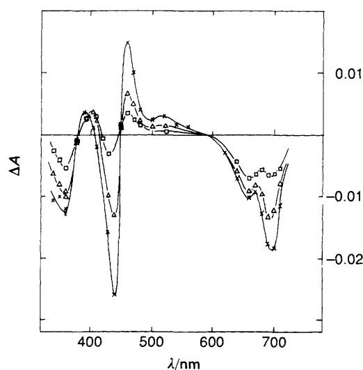
Fig. 8 Nanosecond differential spectrum of the excited ZnP(N^+C_{22})_4/AIClPcTS^{4-} dimer. \lambda_{exc} = 532 nm, 150 homolayers
