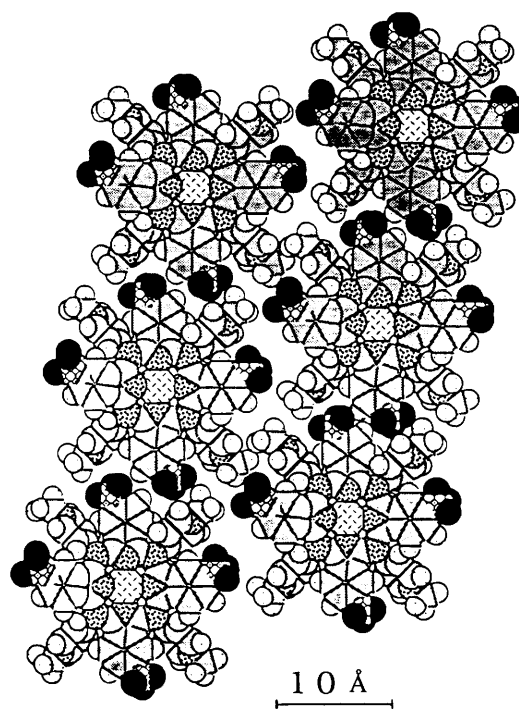
Fig. 2 Molecular model of a two-dimensional packing of the semi-amphiphilic heterodimers on the water subphase and within the LB films. A top view
