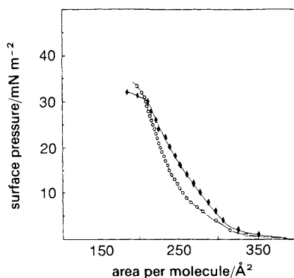
Fig. 1 Pressure vs. area isotherms of the semi-amphiphilic heterodimers on pure water. ◆, \text{ZnP}(\text{N}^+\text{C}_{22})_4/\text{CuPcTS}^{4-} ; ○, \text{ZnP}(\text{N}^+\text{C}_{22})_4/\text{AlPcTS}^{4-}
