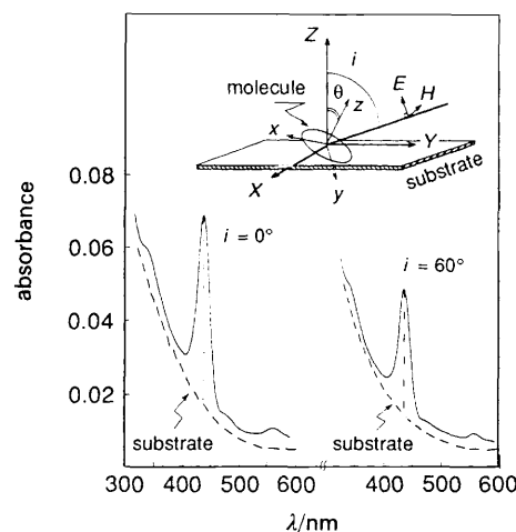
Fig. 4 Soret band intensity for two incident angles i = 0 and 60^\circ under linearly polarized light. H = magnetic field, E = electric field. \theta is the tilted angle between the dimer plane and the substrate plane (two layers)
