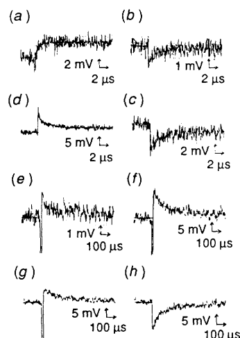
Fig. 9 Microsecond kinetics traces at different wavelengths: (a) 410 nm, I_0 = 450 mV; (b) 440 nm, I_0 = 57 mV; (c) 460 nm, I_0 = 350 mV; (d) 680 nm, I_0 = 122 mV; (e) 410 nm, I_0 = 980 mV; (f) 460 nm, I_0 = 905 mV; (g) 520 nm, I_0 = 910 mV; (h) 700 nm, I_0 = 850 mV
