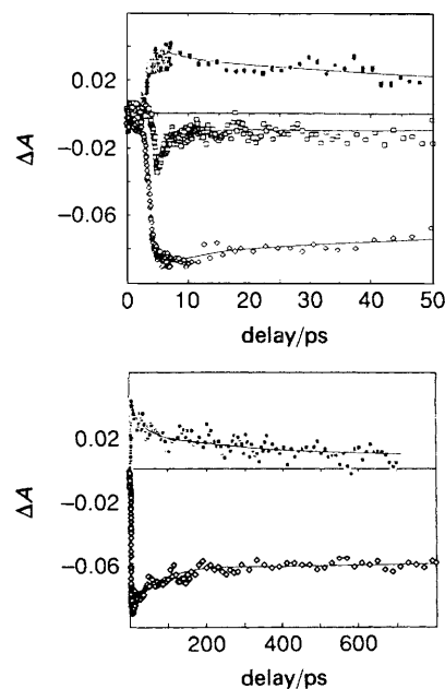
Fig. 7 Picosecond kinetics traces at different wavelengths/nm: \square , 455; \blacksquare , 520; \diamond , 700
