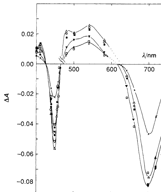
Fig. 6 Picosecond differential absorption spectrum of the excited \text{ZnP}(\text{N}^+\text{C}_{22})_4/\text{AlClPcTS}^{4-} dimer in LB homolayers; the number of layers was, respectively, 150 and 300 in the UV (400–460 nm) and visible region (460–750 nm). t/\text{ps} : \times , 0; \bullet , 0.45; \Delta , 0.95; \circ , 1.45; \blacksquare , 1.95; \blacktriangledown , 4.95; \square , 25. \lambda_{\text{exc}} = 565 \text{ nm}
