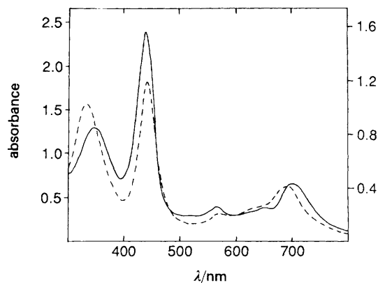
Fig. 5 Absorption spectrum of: (---) \text{ZnP}^{4+}/\text{AlClPcTS}^{4-} in water, c = 10^{-5} \text{ mol dm}^{-3} , optical pathlength = 1 cm (right ordinate); (—) LB film of \text{ZnP}(\text{N}^+\text{C}_{22})_4/\text{AlClPcTS}^{4-} dimer (220 layers) alternated with \omega -tricosenoic acid (220 layers) (left ordinate)
