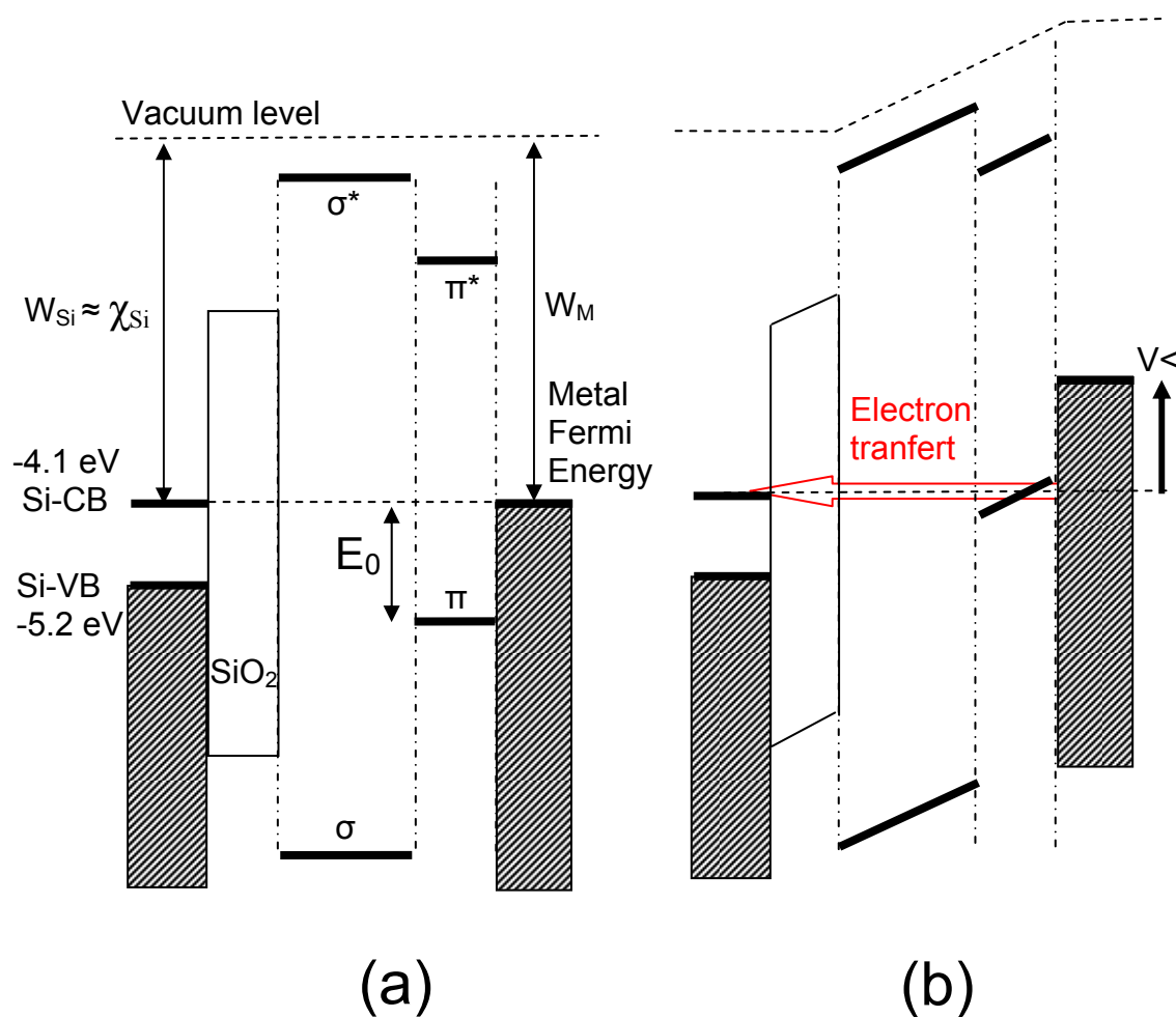
Figure 10. Schematic representation of the energy diagram of the silicon (covered by native \text{SiO}_2 ) /alkyl- \pi group/metal junction: (a) At 0 V; (b) at a negative bias on the metal electrode for which a resonant electron transfer can occur through the \pi -level from the metal to the empty states of the Si CB, for simplicity we assumed a linear potential drop through the SAM.
