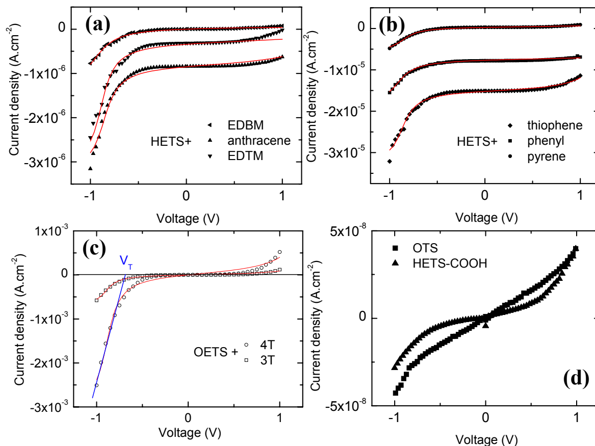
Figure 8. Typical current density - voltage characteristics of the Si/σ-π/Al junctions: (a) HETS/EDBM (◄), HETS/anthracene (▲), HETS/EDTM (▼); (b) HETS/phenyl (■), HETS/pyrene (●), HETS/thiophene (◆); (c) OETS/3T (□), OETS/4T (○). Some curves are vertically shifted for clarity. Red solid lines are fits by equation (2). For the OETS/4T, we show the determination of threshold voltage for rectification, V_T , which is defined as the intercept between a linear fit (dotted line) of the current at high negative voltages and the x-axis. (d) The current-voltage characteristic for the OTS and COOH-terminated HETS (i.e. without π end group) are presented as reference.
