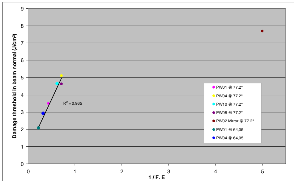
Fig. 10. Damage performance at 1.053 μm, 77.2° or 64.05° of incidence, TE polarization, 500 fs versus 1/E² maximum on four different MLD samples and a mirror (PW02).
