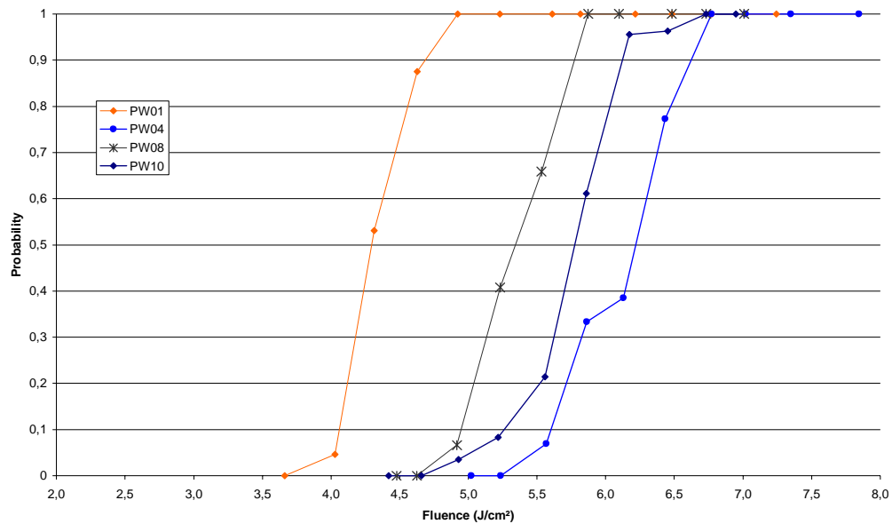
Fig. 8. Damage performance at 1.053 \mu\text{m} , 77.2°, TE polarization, 500 fs of 4 MLD samples
