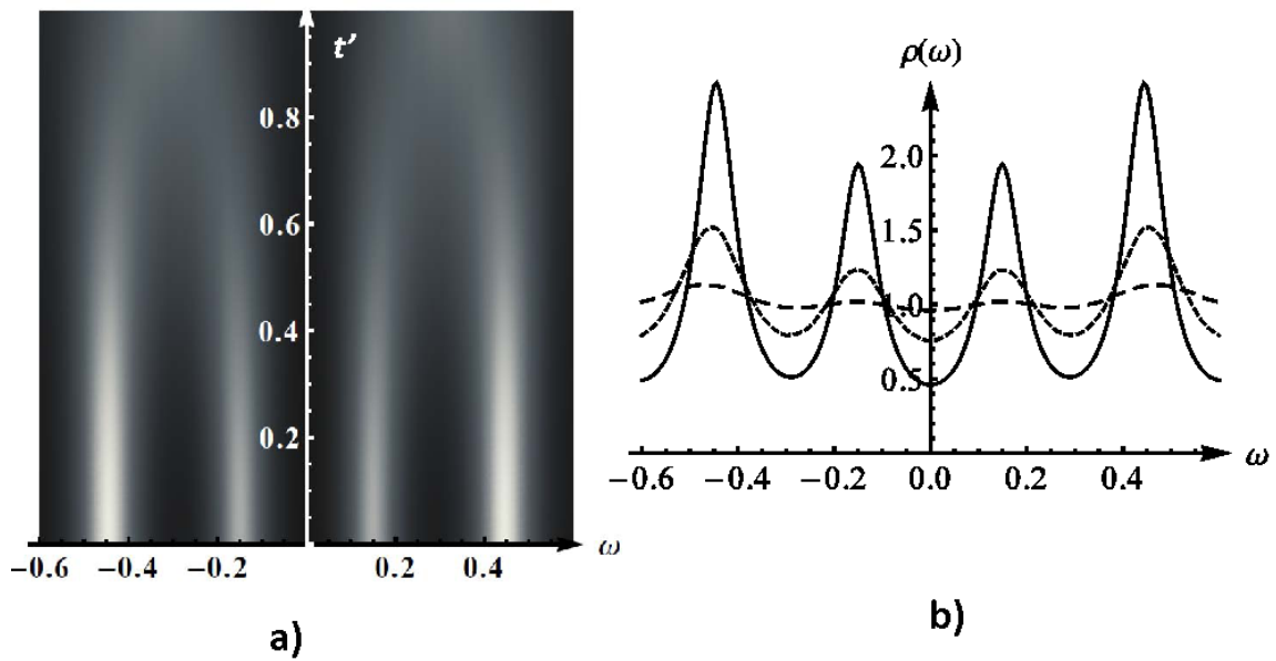
Figure 4: a) Two-dimensional plot of the DOS on the site S + N/2 as a function of energy and coupling with the leads b) The DOS on one central site as a function of energy for three different values of the coupling with the leads: t' = 0 (full line), t' = 0.5 (dashed line), and t' = 0.8 (large-dashed line). The hopping parameter in the bulk was taken to be t = 1 . The other parameters are \delta = 0.05 , S = 100 , and N = 20 .
