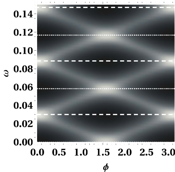
Figure 14: Dependence of the DOS on the site S + 1 on energy and the phase difference between the SCs. The parameters N = 100 , S = 20 , \Delta = 0.3 , t = t' = 1 , and \delta = 0.01 are chosen so that we are in the Andreev limit. The dashed lines and the dotted lines describe the NBS spectrum for N = 100 and N = 101 respectively.
