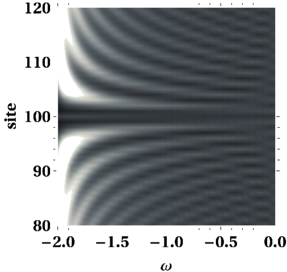
Figure 2: The density of states as a function of position and energy in a one-dimensional chain with a single impurity. We have taken t = 1 , V_0 = 1 , and \delta = 0.04 .
