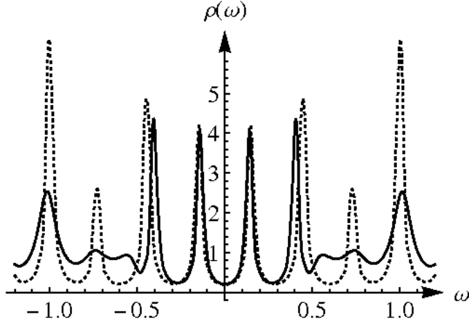
Figure 7: The DOS as a function of energy for a system with S = 200 , N = 20 , and \delta = 0.02 . The site for which the DOS is evaluated is S + N/2 = 210 . The hopping term t has been set to 1. The coupling with the leads is set to zero for the dotted line, and to t' = 0.5 for the full line. The SC gap is set to \Delta = 0.5 .
