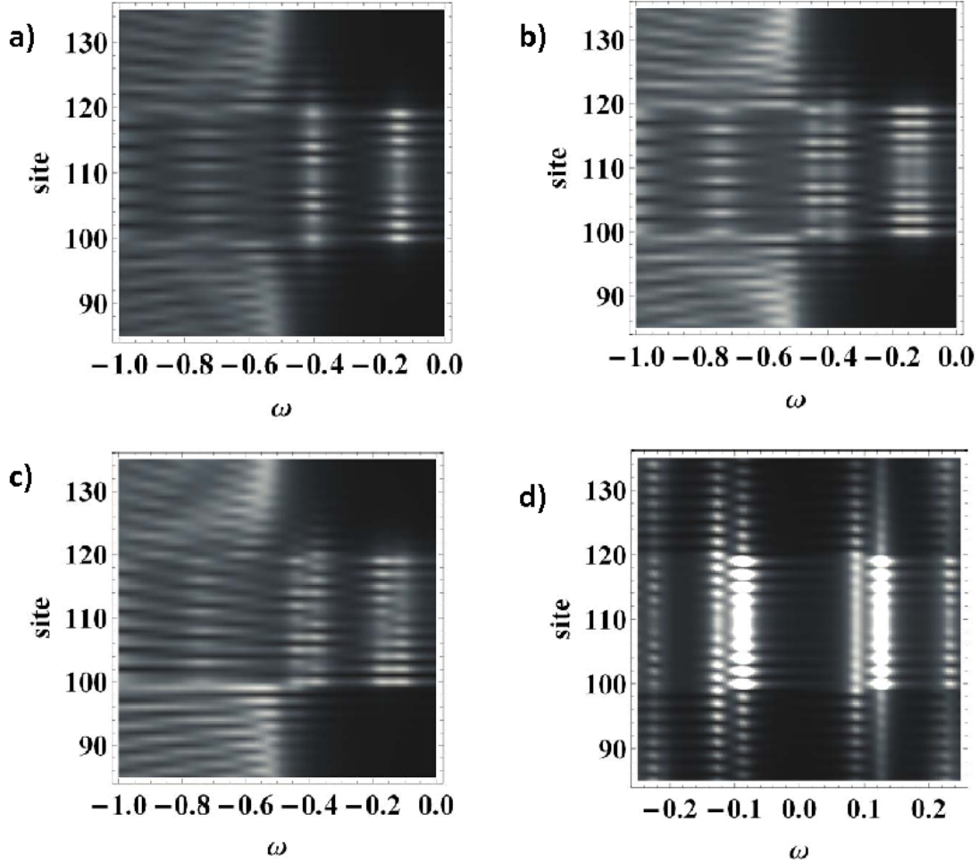
Figure 12: The DOS as a function of energy and position. In a) the parameters are identical to the ones in Fig. 11, in b) we have introduced a non-zero flux \phi = 2\pi/3 , in c) the coupling with the leads is asymmetric, t'_R = 0.25 , t'_L = 0.75 , while in d) the gate voltage is non-zero \mu = -0.05 , \Delta = 0.2 and \delta = .01 .
