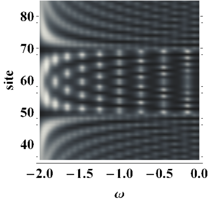
Figure 3: The DOS as a function of position and energy in a one-dimensional chain with two impurities. We have taken S = 50 , N = 20 , \delta = 0.05 , t' = 0.2 , and t = 1 .
