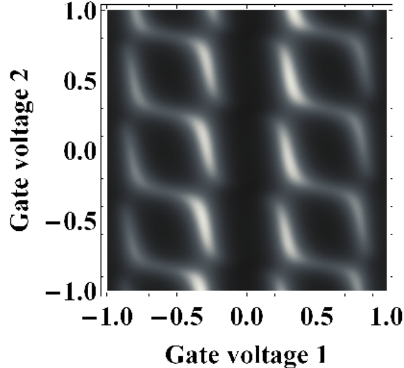
Figure 6: The DOS on one dot as a function of the two gate voltages on the two dots. The parameters are t = 1 , t_{inter-dot} = 0.3 , t' = 0.5 .
