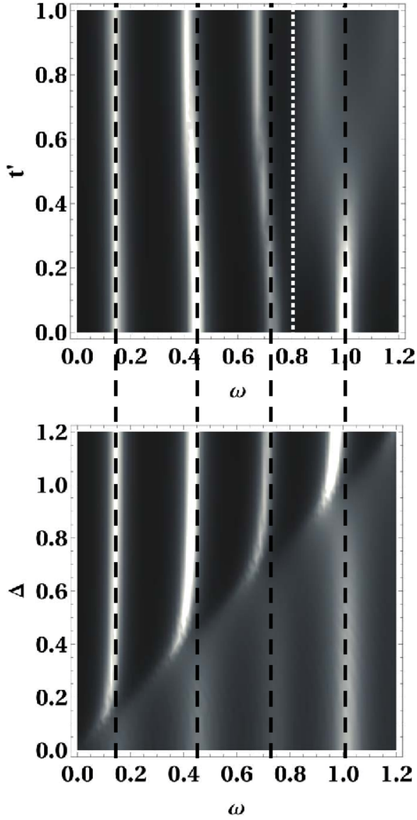
Figure 8: The DOS as a function of energy on the x-axis, and, on the y-axis, the coupling to the leads ( t' ) (top panel) and the superconducting gap ( \Delta ) (bottom panel). The coupling with the leads is assumed to be symmetric. We have taken \Delta = 0.8 for the upper plot, and t' = 0.5 for the lower plot, S = 150 , N = 20 , and \delta = 0.02 . The site for which the DOS is evaluated is S + N/2 = 160 . The hopping term t has been set to 1. The positions of the NBS are given by the black dashed lines, while the gap is indicated in the upper panel by the white dotted line.
