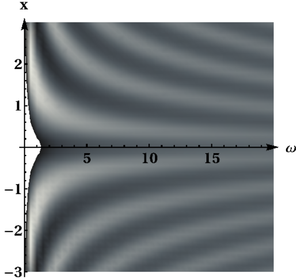
Figure 5: The DOS as a function of position and energy in a one-dimensional chain with a single impurity. The impurity potential is set to V = 1 .
