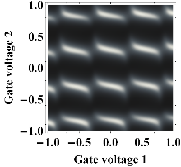
Figure 13: The DOS on one dot as a function of the two gate voltages on the two dots. The parameters are set to t = 1 , t' = 0.5 , t_{inter-dot} = 0.5 , \Delta = 0.5 , and \delta = 0.04 .
