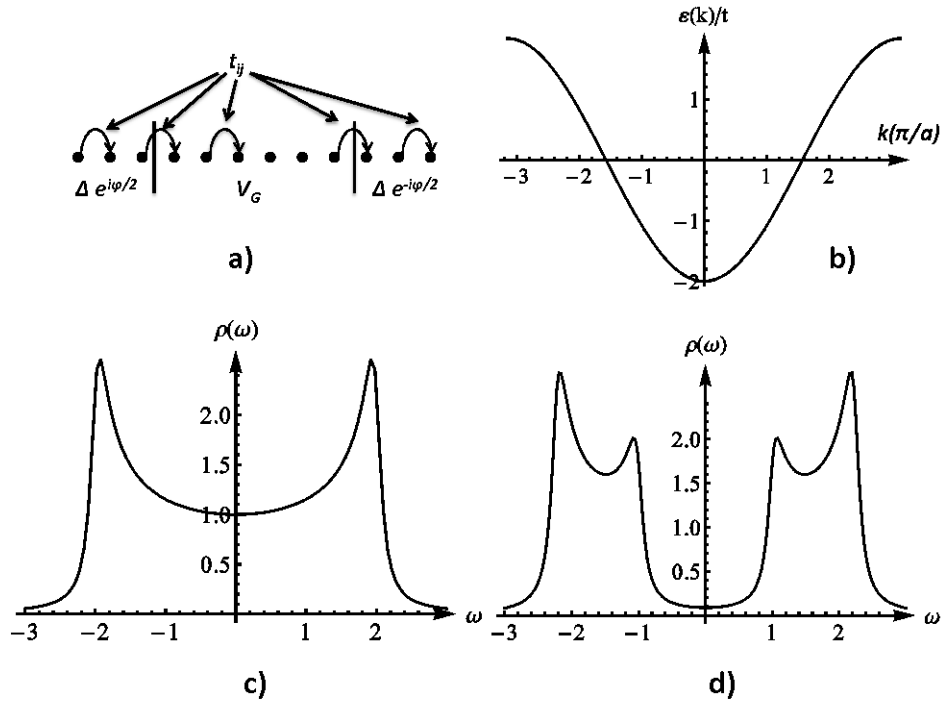
Figure 1: a) One-dimensional chain. b) The energy dispersion for the infinite uniform system and (c) the corresponding density of states d)The density of states when the gap is non zero ( \Delta = 1 ). In c) and d) we have set t = 1 , and we have performed the calculations for a uniform system of 100 sites, with a roughly large \delta = 0.1
