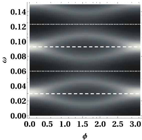
Figure 15: Dependence on the DOS on energy and phase for a N = 100 link, when the system is no longer in the Andreev limit. This is achieved by using the same parameters as the ones in Fig. 14, and increasing the gap to \Delta = 2 . We can see that the amplitude of the variation with the phase is reduced, and gaps open at \phi = \pi . Same as above, the dashed lines and the dotted lines describe the NBS spectrum for N = 100 and N = 101 respectively.
