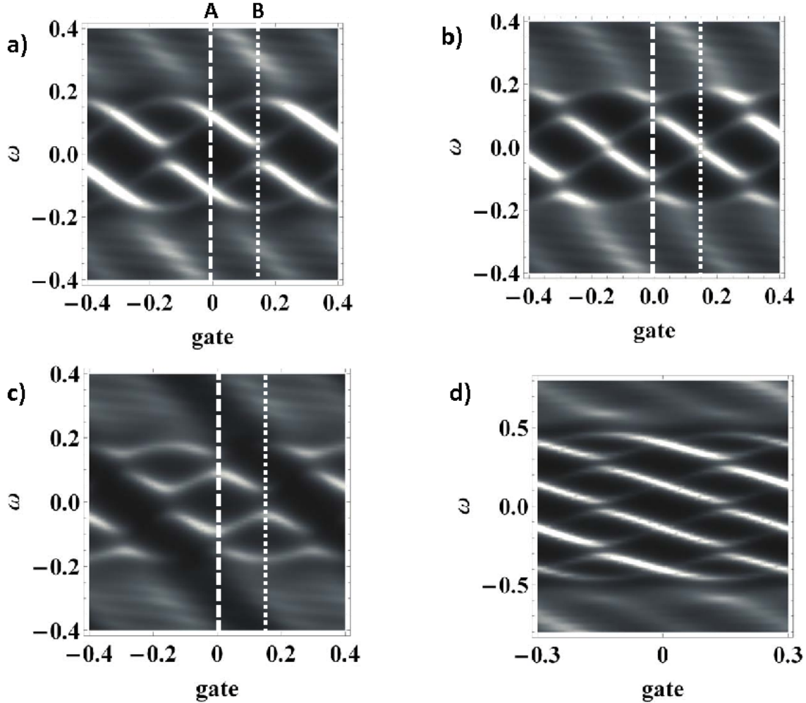
Figure 9: The DOS as a function of energy and gate voltage. We have set a) N = 20 , S = 100 , t = 1 , t' = 0.5 , \Delta = 0.2 , and \delta = 0.02 ; b) same as in a) plus a phase difference between the two SC of 2\pi/3 ; c) same as a) plus an asymmetric coupling of the link with the two SCs, t'_R = 0.25 , t'_L = 0.75 ; d) same parameters as in a) except for \Delta = 0.5 . The white dashes lines A and B correspond to a gate voltage of \mu = 0 and respectively \mu = \pi/N .
