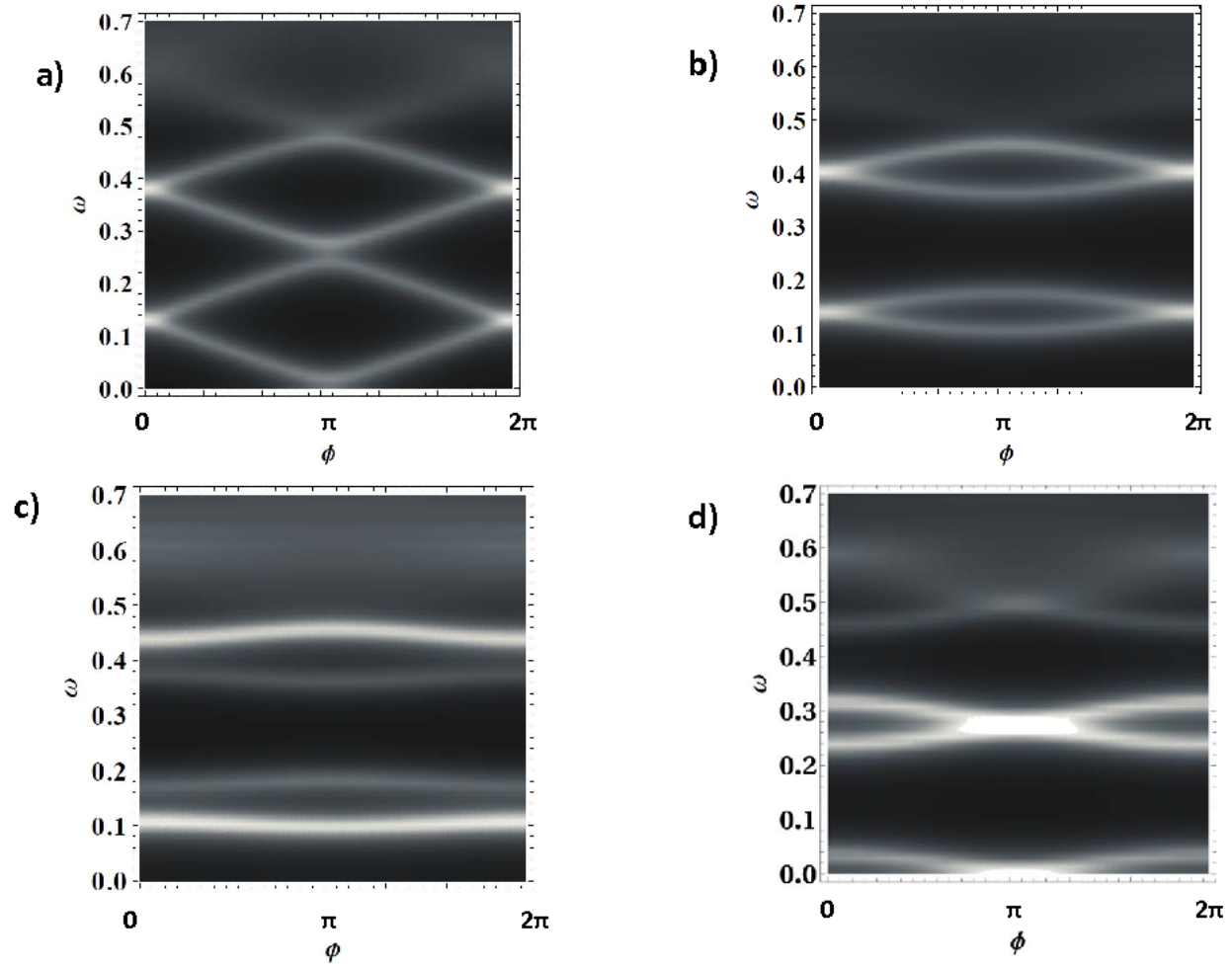
Figure 10: The DOS as a function of energy and phase difference on the site S+N/2 . The parameters are S = 100 , N = 20 , t = 1 , \delta = 0.02 , \Delta = 0.5 , and a) t' = 1 , b) t' = 0.5 , c) t'_R = 0.25 , t'_L = 0.75 d) same parameters as a) but for non-zero gate voltage \mu \approx \pi/(N + 1) . The spectra in a), b) and c) correspond to the line A in Fig. 9, and the spectrum in d) corresponds to the line B in Fig. 10.
