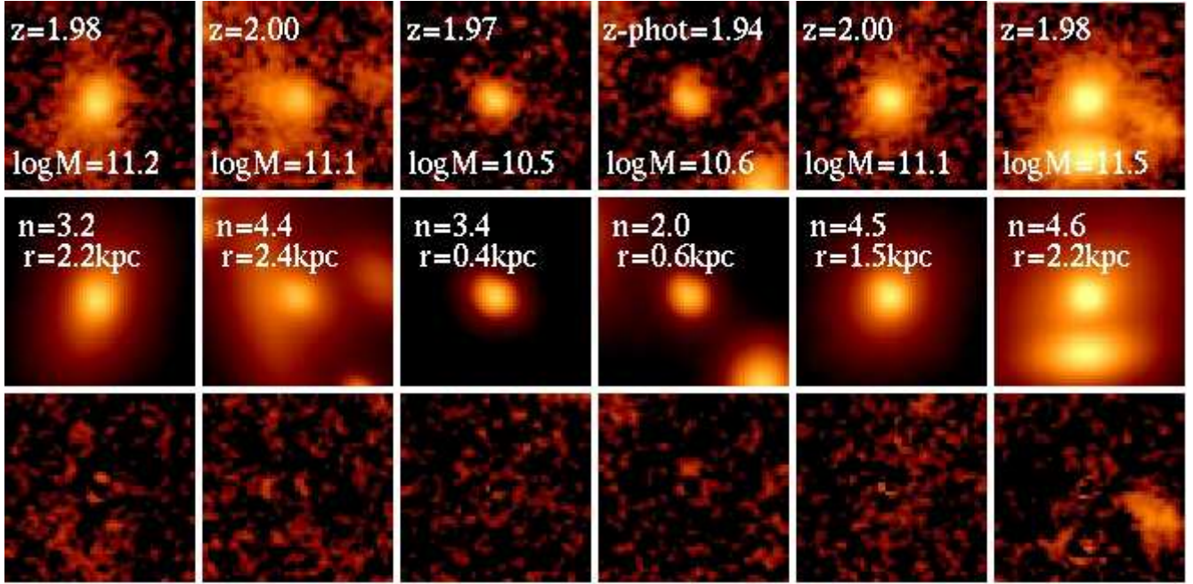
FIG. 10.— WFC3 F140W cutouts of the 6 massive passive members with a n_{Sersic} > 2 . The top, middle, and bottom panels show the image, model, and residual for these six sources. Cutout size is 3'' , or \sim 26 kpc at z=2 .
