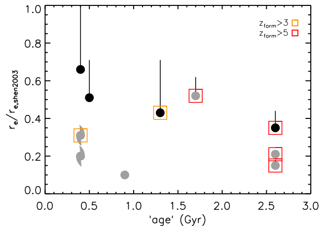
FIG. 13.— The “age” vs size evolution factor for the \geq 10^{11} M_{\odot} cluster (black symbols) and field (gray symbols) passive early-types (see Figure 12, and the text for the definition of the plotted quantities). Black lines are not errors on the size determination (see Figure 12), but show the offset in evolution factor if using M05 rather than BC03 stellar masses, for the same local reference.
