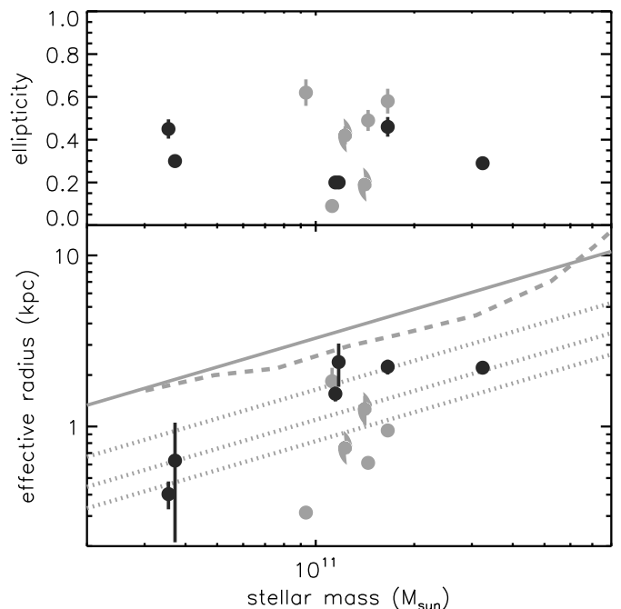
FIG. 12.— The ellipticity and effective radius as a function of stellar mass, for cluster (black) and field (gray, 1.5 < z < 3 ) passive early-type galaxies in the probed area. Two field galaxies with 1.5 < n_{Sersic} < 2 are included, and are shown as spiral symbols. In the bottom panel, the solid and dashed lines show, respectively, the local determination of the stellar-mass size relation by Shen et al. (2003) for early-type galaxies, and by Valentinuzzi et al. (2010) for nearby cluster early-types. The dotted lines show for reference the Shen et al. (2003) relation scaled by a factor 2, 3, and 4 in size.
