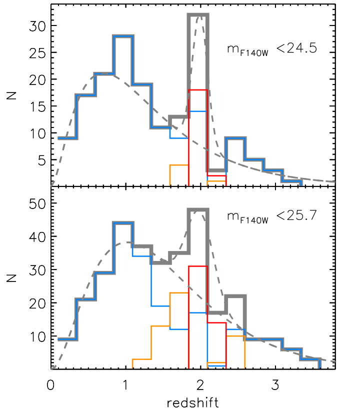
FIG. 2.— The redshift distribution in the cluster field. Gray lines show the distribution (of photometric redshifts, or spectroscopic where available) of all sources in the target area down to m_{140} = 24.5 and 25.7 (upper and lower panel, respectively). The contributions of galaxies identified as interlopers, “possible” and “likely” cluster members, as described in the text, are shown as blue, orange and red lines, respectively. Dashed gray lines in both panels show a modeling of the redshift distribution in this field, with and without the cluster contribution (see text).
