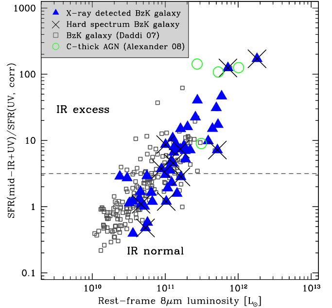
FIG. 1.— Ratio of star-formation rates (SFRs; mid-IR and extinction-corrected UV) for the z \approx 2 galaxies studied by Daddi et al. (2007a,b) versus rest-frame 8 \mu\text{m} luminosity. Triangles correspond to X-ray detected BzK galaxies, crosses indicate the BzK galaxies with hard X-ray spectral slopes (heavily obscured AGNs; see Fig. 2), open squares correspond to the X-ray undetected BzK galaxies, and the open circles correspond to the spectroscopically identified (optical and mid-IR wavelengths) Compton-thick AGNs at z \approx 2 from Alexander et al. (2008) in the 2 Ms Chandra Deep Field-North survey (Alexander et al. 2003). The threshold between IR excess and IR normal galaxies defined by Daddi et al. (2007a,b) is indicated by the dashed line.
