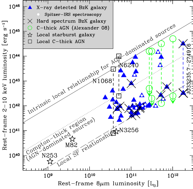
FIG. 3.— Rest-frame 2–10 keV luminosity versus rest-frame 8 \mu\text{m} luminosity. The symbols have the same meaning as in Figs. 1 & 2; in addition, the small filled circles show the X-ray detected BzK galaxies with Spitzer -IRS spectroscopy. The X-ray– 8 \mu\text{m} luminosity ratio for local starburst galaxies (long-dashed line) is taken from the X-ray– 12 \mu\text{m} luminosity ratio of Krabbe et al. (2001) and converted to 8 \mu\text{m} assuming the M 82 spectral energy distribution. The intrinsic X-ray– 8 \mu\text{m} luminosity ratio for local AGNs (solid line) is taken from Lutz et al. (2004) and converted to 8 \mu\text{m} , assuming the AGN-dominated galaxy NGC 1068; the dotted line indicates the observed X-ray– 8 \mu\text{m} luminosity ratio predicted for Compton-thick AGNs. The rest-frame 8 \mu\text{m} luminosity for the X-ray detected BzK galaxies is calculated from the 24 \mu\text{m} flux density, with small K -corrections applied (see Daddi et al. 2007a), while the rest-frame 8 \mu\text{m} luminosity for the local starburst galaxies is calculated using the mid-IR spectroscopy of Rigopoulou et al. (1999) and Lutz et al. (2003). The vertical dashed lines indicate the difference between the observed and intrinsic X-ray luminosity for the z \approx 2 Compton-thick AGNs from Alexander et al. (2008) and Feruglio et al. (2011); the intrinsic X-ray luminosity constraint for J033235.7–274916 is from Feruglio et al. (2011), which is one of the heavily obscured AGNs in our sample.
