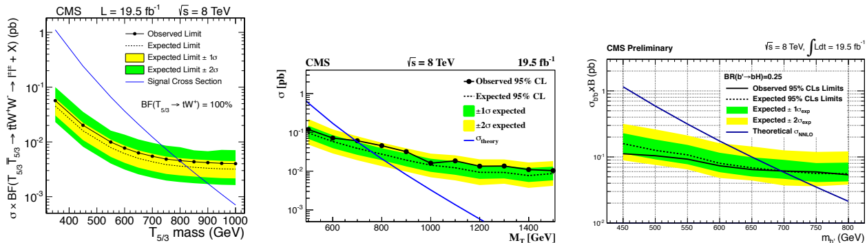
Figure 6: CMS bounds on spin 1/2 top partners after run 1. Left: the bound on the charge 5/3 top partner from [204], middle: the bound on the charge 2/3 singlet from [205], right: the bound on the charge -1/3 singlet bottom partner from [206].
