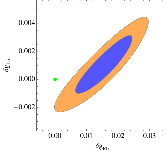
Figure 3: Best fit region for the Z\bar{b}b couplings from [101] favoring small positive \delta g_{Rb} . The SM is represented by the green point.
