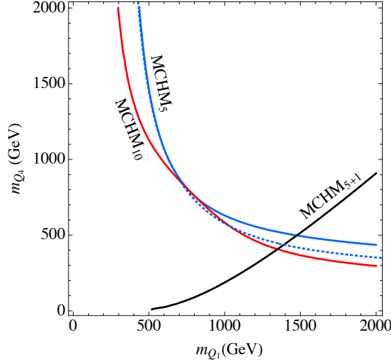
Figure 1: Masses of the top partners Q_1 and Q_4 that reproduce the Higgs mass m_h = 125 GeV for v^2/f^2 = 0.2 , from [86]. The different lines correspond to different SO(5) embeddings for the top quark. In blue q_L, t_R \in \mathbf{5} , in red q_L, t_R \in \mathbf{10} (with Q_1 \rightarrow Q_6 ) and in black q_L \in \mathbf{5} and t_R \in \mathbf{1} .
