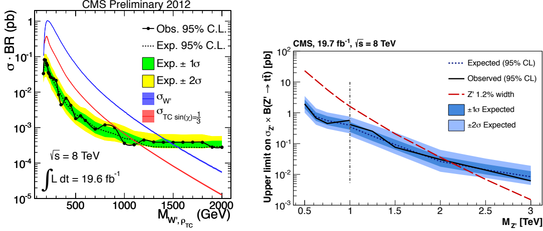
Figure 5: Preliminary CMS bounds from run 1 of the LHC on the production of spin 1 resonances. Left panel: bound on \rho^\pm using decays to WZ , from [184]. Right panel: bound on the KK gluon decaying to t\bar{t} , from [186]. Note that the dashed curve is for a Z' , the KK gluon bound from the same plot is around 2.5 TeV.
