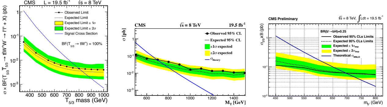
Figure 6: CMS bounds on spin 1/2 top partners after run 1. Left: the bound on the charge 5/3 top partner from [204], middle: the bound on the charge 2/3 singlet from [205], right: the bound on the charge -1/3 singlet bottom partner from [206].
