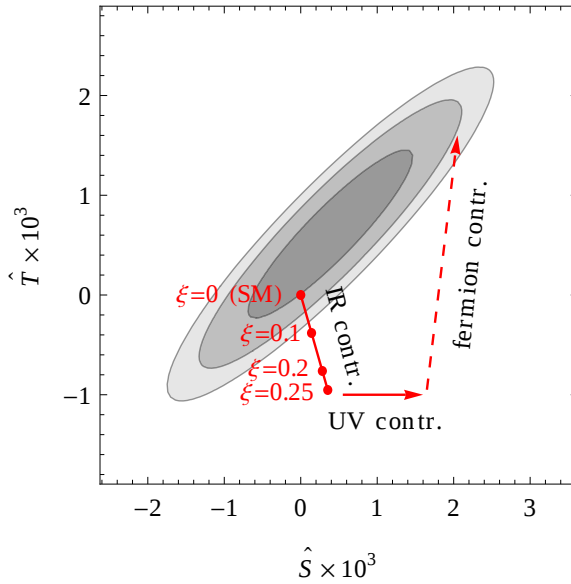
Figure 2: Confidence level contours (at 65%, 95% and 99%) for \hat{S} and \hat{T} from [97]. The IR contributions alone would imply \xi = v^2/f^2 \lesssim 0.1 .
