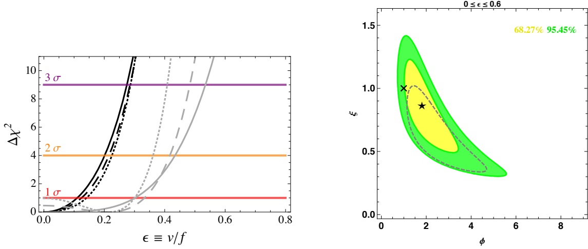
Figure 4: Higgs fits from [129] (left panel) and [139] (right panel). Left panel: Fit to v/f for the MCHM with (black) or without (gray) including electroweak precision data, with n_\psi = 0 (solid), n_\psi = 1 (dashed), and n_\psi = 2 (dot-dashed). Right panel: Fit to \xi = v^2/f^2 and c_{\gamma\gamma}/\xi from Higgs data, with \epsilon \equiv \gamma_\psi marginalized in the range 0 \leq \epsilon \leq 0.6 . The star is the best-fit point, while the cross corresponds to Higgs-like dilaton limit.
